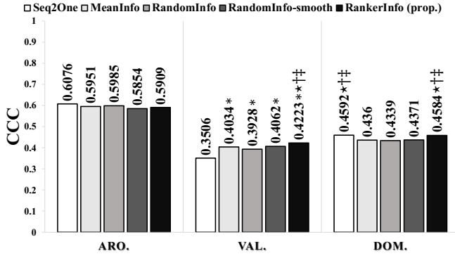
(b) Results on the MSP-IMPROV corpus
