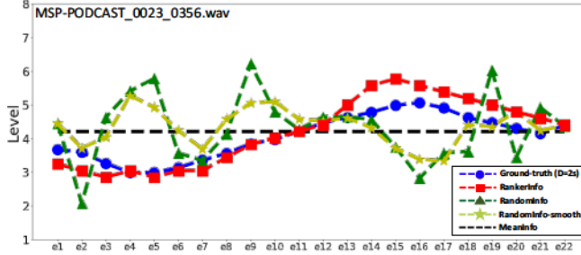
Fig. 4. Example of retrieved curves for valence based on different approaches. The figure also provides the ground-truth curve from the time-continuous annotations provided in the MSP-Conversation corpus.
