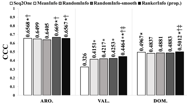
(a) Results on the IEMOCAP corpus
