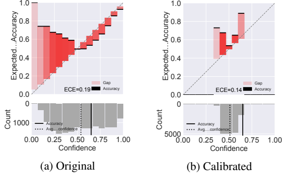
Figure 2: Confidence versus accuracy diagrams of predictions for a model trained with \mathcal{L}_{P+CB} ( \alpha = 0.2 ) for happiness before and after the multi-label TS calibration method. The grey bars are the distribution of the data based on confidence.
