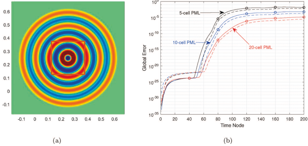
FIGURE 4. Example 4: The global errors obtained on a 100 \times 100 mesh with a point wave source. (a) Illustration of domains \Omega_G and \Omega_L . (b) The global errors obtained with three different PML thicknesses.
