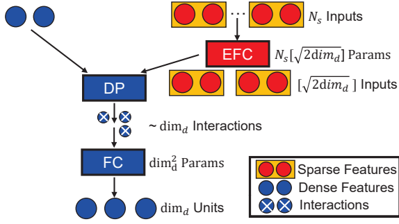
Figure 4: Operator-balancing interaction inserts a simple EFC layer before Dot-Product to ensure linear parameter consumption and balance building operators.
