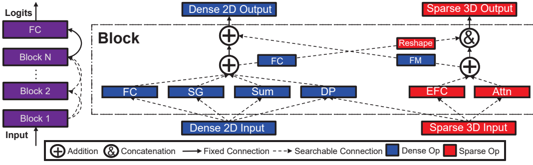
Figure 1: Overview of NASRec search space. NASRec search space enables a full architecture search on building operators and dense connectivity. Here, “blue” blocks produce a dense output, and “red” blocks produce a sparse output.
