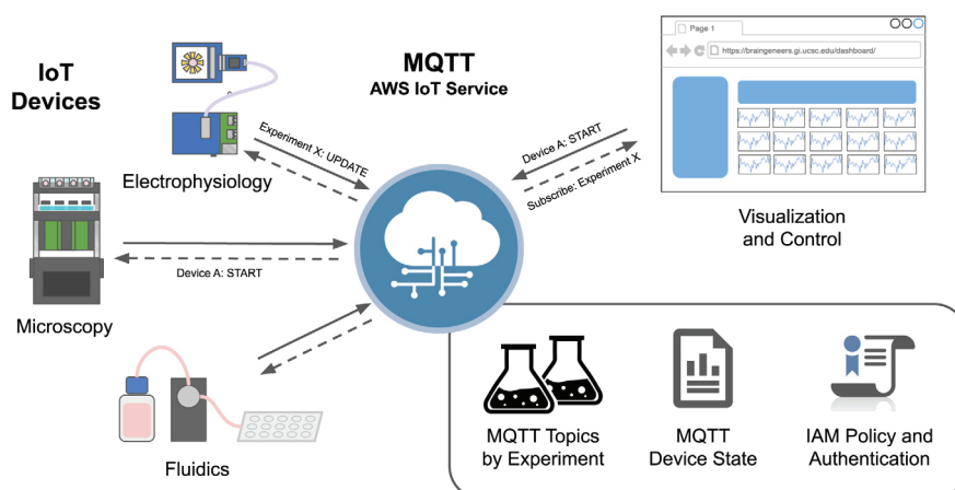
Fig. 2. Inter-device MQTT message broker. The MQTT message broker provides integration and control over multiple internet-connected instruments. The functionality supports clients , data acquisition modules or software applications, to connect and subscribe to topics set by a publisher , such as the user interface (UI), with the proper authentication protocols. By doing so, clients subscribed to the topic will be informed of the state of each data acquisition module (e.g., start, stop, etc.) and parameter changes throughout an experiment.
