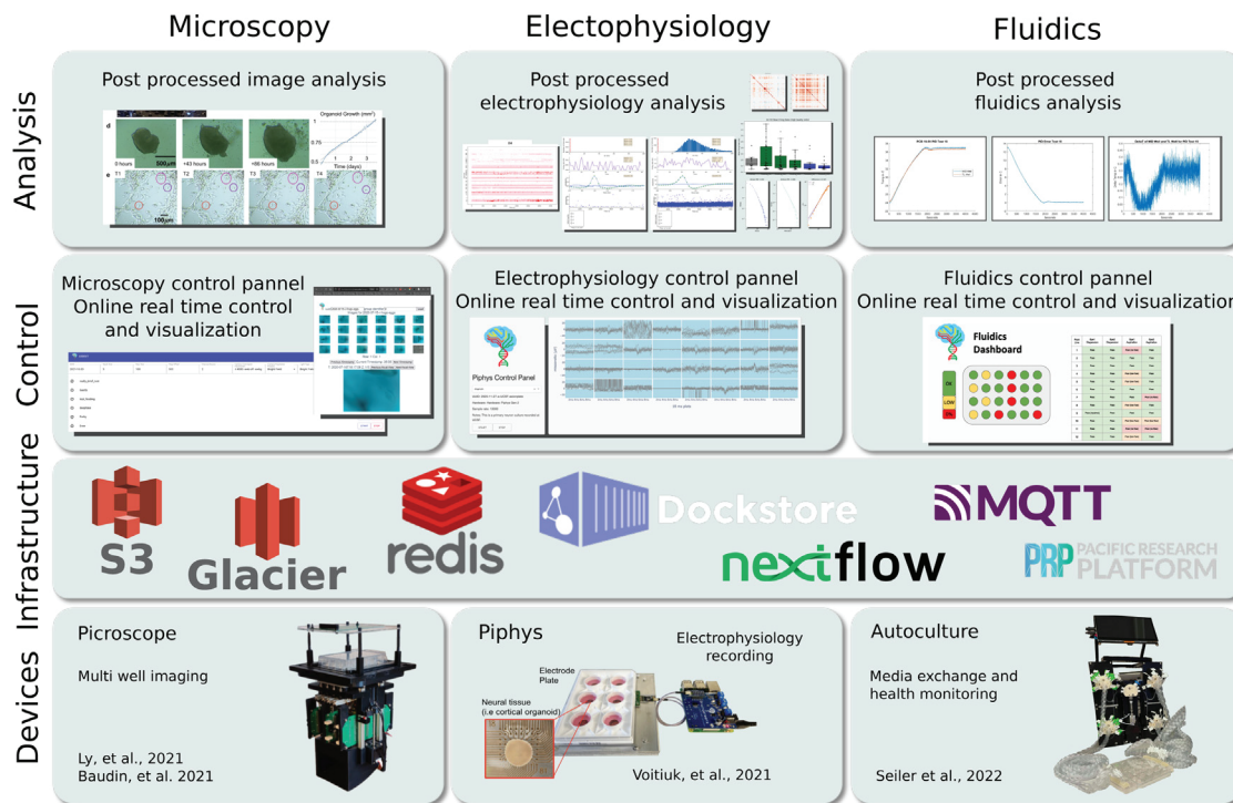
Fig. 6. An outline of existing tools that utilize the IoT Cloud Laboratory platform described in this paper. (Device) shows Picroscope [32,33] for microscopy, Piphys [34] for electrophysiology recording, and Autoculture [35] for fluidic media exchange and liquid biopsy. (Infrastructure) shows the primary suite of tools introduced in Sections 3.2, 3.4 and 3.5. (Control) shows a snapshot of existing web-based control interfaces. These web pages are running on a server in the UCSC Genomics Institute. (Analysis) demonstrates some of the reports produced by workflows that run as data post-processing jobs. “Picroscope” and “Piphys” figures are adapted from Ly et al. [32], Baudin et al. [33], Voitiuk et al. [34].
