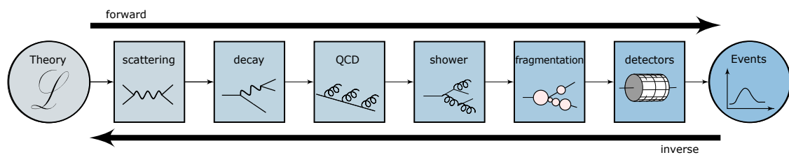
Figure 1: Illustration of the LHC simulation chain. The forward direction is discussed in Secs. 2 and 3, while the inverse simulation is the topic of Sec. 4.
