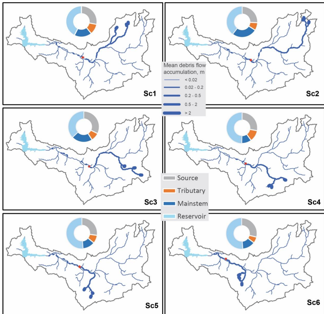
Figure 3. Debris flow accumulation in the Provo River network after the equivalent 30-yr flow simulation under different spatial input distributions (Sc1 to Sc6; initial placement at upstream tributary reaches). The proportions (of total 30,000 m 3 ) of storage in the source location, tributary, mainstem and reservoir are shown by different colors in the circle. The downstream extent of 50% mainstem accumulation is showed by a red mark in the mainstem for each case.
