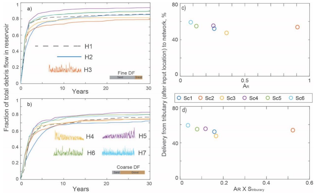
Figure 2. Debris flow sediment transported by all hydrographs for (a) fine and (b) coarse debris flow input. Percentage of input sediment (excluding the input location, gray area in Figure 3) delivered to mainstem after the 30-year simulation against (c) symmetry ratio ( A_R = DA_{tributary} / DA_{mainstem} ), and (d) product of symmetry ratio and tributary slope.
