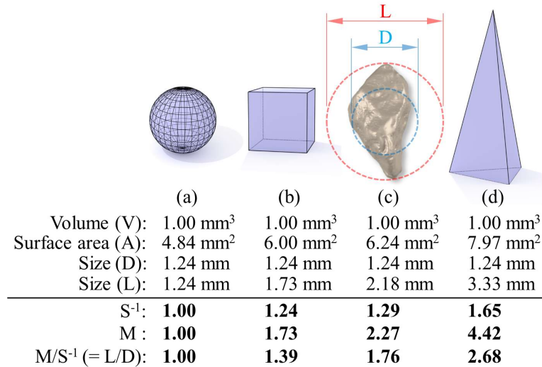
Figure 2. Particle shape evaluated in terms of S^{-1} and M ; (a) Sphere; (b) Cube; (c) a 3D-scanned mineral particle; and (d) Elongated tetrahedron
