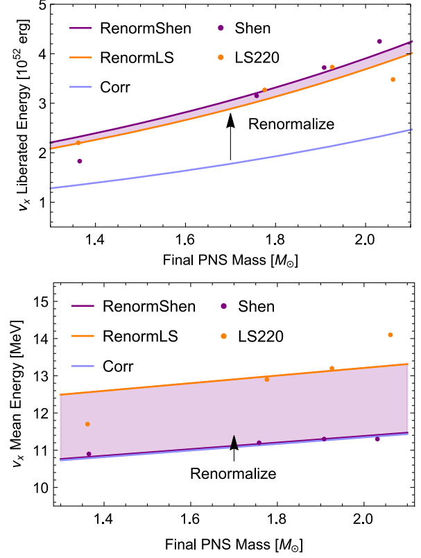
FIG. 10. Same as Fig. 4 but for \nu_\mu . In the bottom panel, the renormalization constant for mean energy is equal to 1 between Corr and RenormShen.
