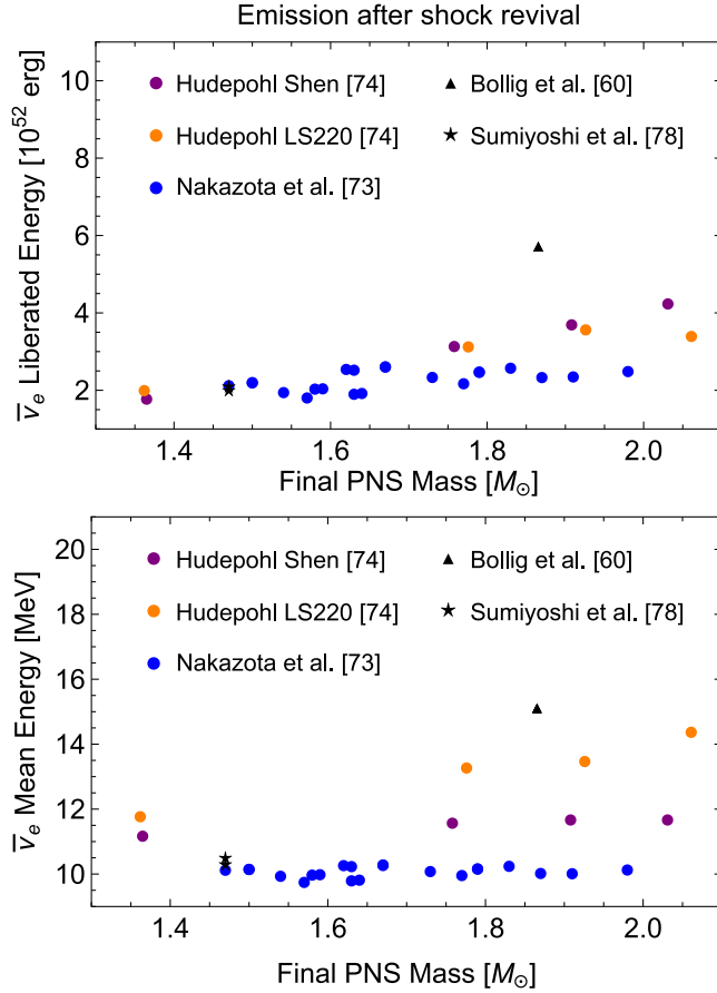
FIG. 1. Comparison of the time-integrated \bar{\nu}_e spectral parameters in the cooling phase of PNS evolution shown against the final baryon mass of the PNS. Here we compare those quantities of the Hudepohl [74], Nakazato [73], Bollig [60], and Sumiyoshi [78] (integrated from shock revival time to the end of simulation time: \sim 10 , 20, \sim 7 , and \sim 60 s, respectively). Their EOSs are the Shen/LS220, Shen, SFHo, and TM1/TM1e, respectively. See text and Table I for details. There are other differences not mentioned here, but these serve to show some dependence of neutrino emission on final PNS mass and hint at systematic differences due to e.g., EOS. More simulation details can be found in Table I.
