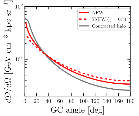
FIG. 1. DM column density dD/d\Omega \equiv \int_{\text{LOS}} \rho_\chi ds versus angle from the GC for NFW and SNFW profiles, as well as the contracted halo of Ref. [51]. Most NuSTAR observations in this work are at moderate distances from the GC, minimizing profile uncertainties. See Sec. IID for further details.
