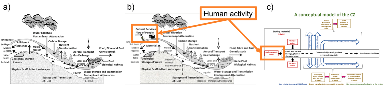
Fig. 6. Critical Zone researchers are increasingly focused on the resilience of the CZ to novel and large-scale anthropogenic perturbations (orange boxes added). a) A conceptual model of the CZ (Banwart et al., 2012 [Fig. 1]) is modified to incorporate the impact of human activity in b) Banwart et al. (2013) [Fig. 1]) at a surficial level. c) Human activity is conceptualized as a primary driver of CZ processes that affect CZ architecture, character, and dynamics (Brantley et al., 2016 [Fig. 1]).
