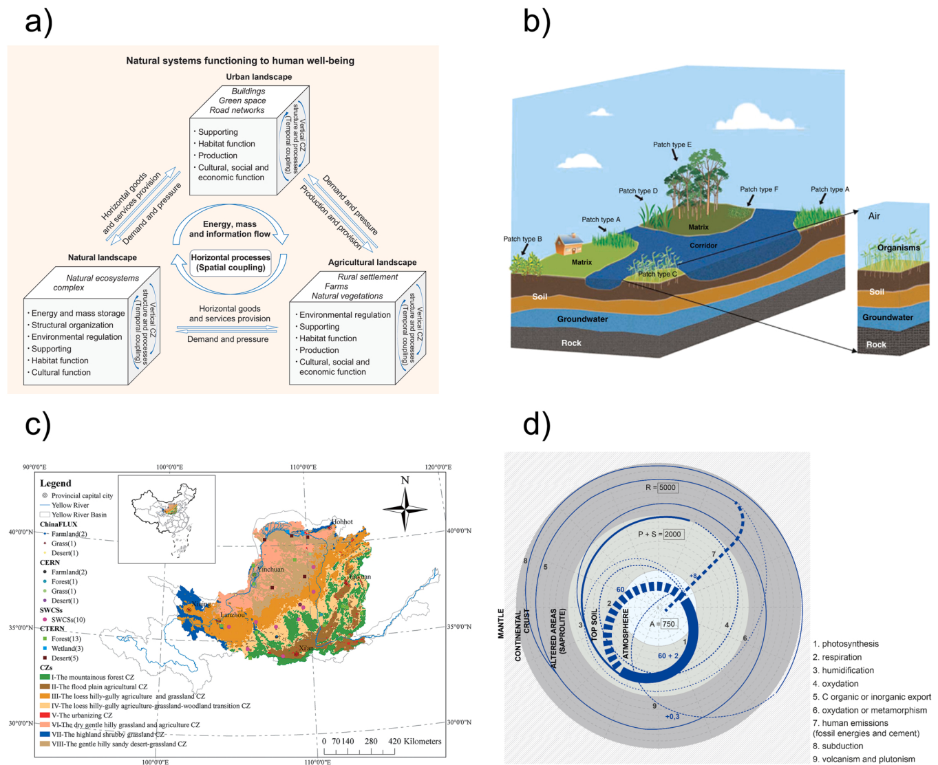
Fig. 10. Emerging trends in Critical Zone research with respect to coupling of research disciplines include: a) new conceptual models connecting the urban and agricultural landscapes to the natural landscape (e.g., Luo et al., 2019 [Fig. 1]), b) new conceptual models accounting for functional patchiness and heterogeneity in the landscape (e.g., Chamorro et al., 2015 [Fig. 7.9]), c) new maps drawn at the regional scale accounting for functional patchiness and heterogeneity in the landscape (Lu et al., 2019 [Fig. 2]), d) new conceptual models of elemental flow through the CZ accounting for human activity (e.g., carbon cycling; Arenes, 2021 [Fig. 12]).
