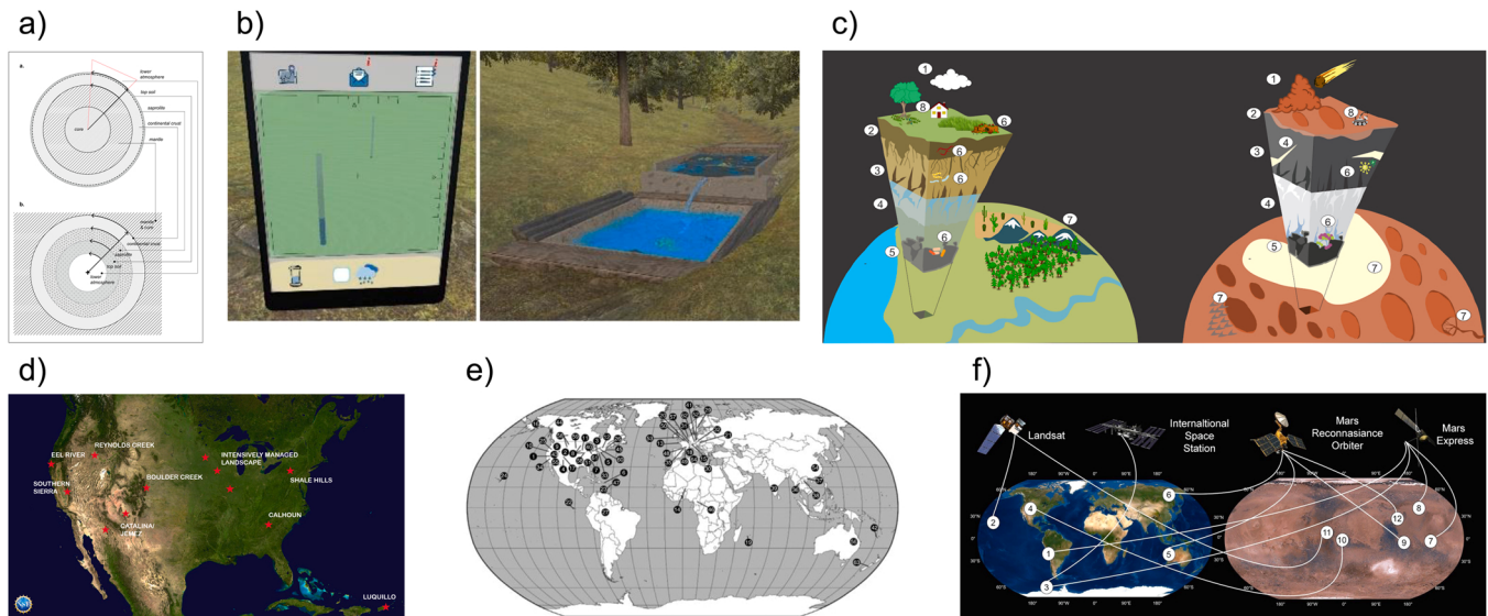
Fig. 8. Emerging trends in Critical Zone research with respect to spatial scale include: a) reconceptualizations of the Critical Zone Observatory (e.g., Arenes et al., 2018 [Fig. 3]), b) study of the CZO in computational spacetime (Sajjadi et al., 2020 [Fig. 5]), and c) study of the CZ on exoplanets (e.g., Mars; Fackrell et al., 2020 [Fig. 1]). The expansion of the CZO network is shown with d) map of the original CZOs across the US (Brantley et al., 2017b [Fig. 2]), e) map of CZOs across the world (Giardino and Houser, 2015 [Fig. 1.2]), and f) map of proposed CZOs across Mars (Fackrell et al., 2020; [Fig. 2]).
