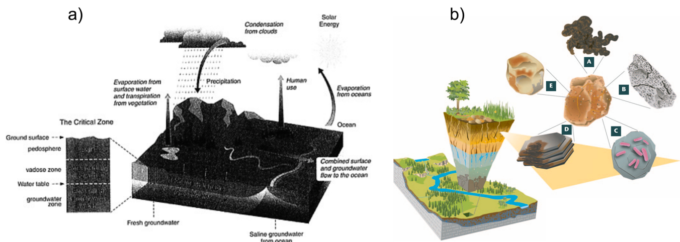
Fig. 1. Conceptual models defining the Critical Zone as a place. a) NRC (2001 [Fig 2.1]) emphasizes the horizontal expanse of the CZ at the scale of the terrestrial surface area of the planet. b) Chorover et al. (2007) [Fig. 1]) emphasize the interactions of the vertical layers of the CZ at the scale of a sub-planetary area.
