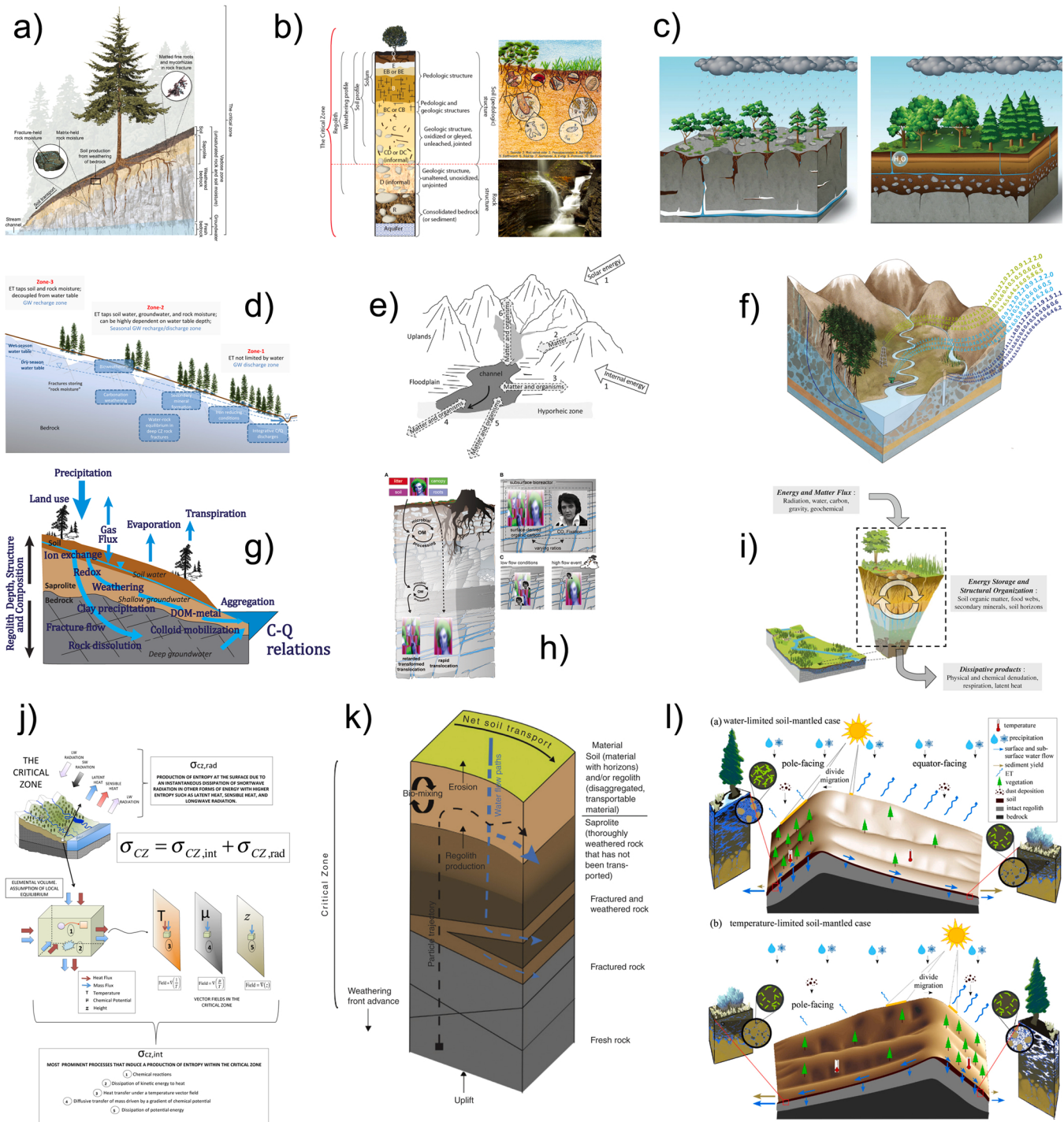
Fig. 5. Conceptual models of unifying threads defining the Critical Zone include: a) plants (Dawson et al., 2019 [Fig. 1]), b) soil (Lin, 2010 [Fig. 1]), c) bedrock (Jiang et al., 2020 [Fig. 1]), d) water (Brooks et al., 2015 [Fig. 3]), e) surface water (Wohl, 2015 [Fig. 9.1]), f) subsurface water (Singha and Navarre-Sitchler, 2021 [Fig. 1]), g) biogeochemical cycling of elements (e.g., nutrients, metals, or carbon; Chorover et al., 2017 [Fig. 1]), h) microorganisms (Kusel et al., 2016 [Fig. 4]), i) energy (Rasmussen et al., 2011 [Fig. 1]), j) entropy (e.g., thermodynamic and information; Quijano and Lin, 2014 [Fig. 2]), k) mineral weathering (Pope, 2015 [Fig. 4.1]), and l) measurement of slope aspect (Pelletier et al., 2018 [Fig. 4]).
