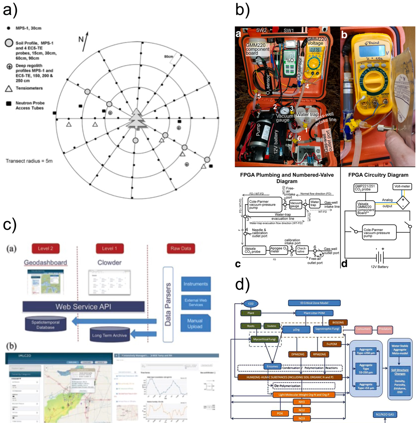
Fig. 3. Novel sensing methods and information technologies developed at different Critical Zone Observatories include a) extensive sensor networks at the Southern Sierra CZO (O'Geen et al., 2018 [Fig. 8]), b) Field Portable Gas Analyzers at the Calhoun CZO (Brecheisen et al., 2019b [Fig. 2]), c) a data management system at the Intensely Managed Landscapes CZO (Wilson et al., 2018 [Fig. 8]), and d) a conceptual model (CZ Integrated Model) of carbon and nutrient flows, which incorporates a numerical model (Carbon dynamics and Aggregate STability [CAST]) of soil aggregate formation and degradation processes, at multiple CZOs (Banwart et al., 2012 [Fig. 11]).
