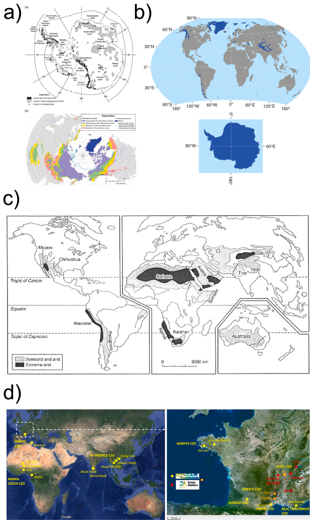
Fig. 2. Diverse and distant biomes across the Critical Zone include a) permafrost (Rowley et al., 2015 [Fig. 13.2]), b) glaciers (Gamache et al., 2015 [Fig. 12.2]), c) deserts (Tchakerian and Pease, 2015 [Fig. 14.1]), and d) intermittent rivers and ephemeral streams (Fovet et al., 2021 [Fig. 1]).
