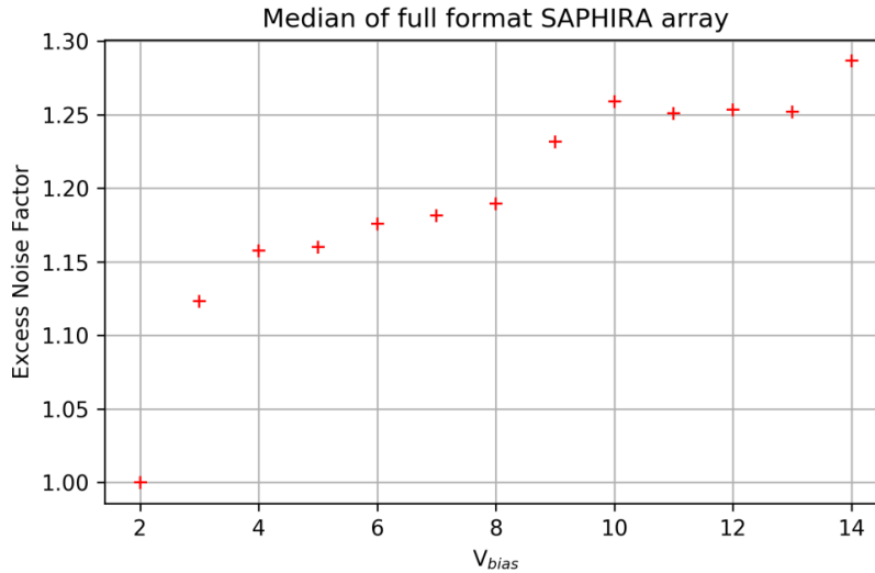
Figure 6: The median excess noise factor across the array as a function of applied bias voltage. There is a more scatter in the excess noise measurement after a bias voltage of 8V. It is possible this is a result of having fewer points within the Poisson-dominated regime of the PTCs for these trials, and therefore, less accuracy in our slope measurements.
