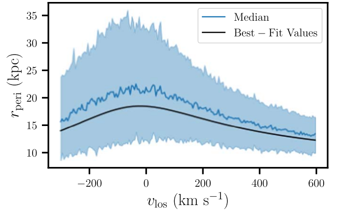
Figure 8. Predicted orbital pericenter ( r_{\text{peri}} ) across a range of possible line-of-sight velocities ( v_{\text{los}} ) for Boötes V. The black line uses the median values for the proper motion and distance, whereas the blue line and bands are from MCMC sampling of the proper motion and distance errors.
