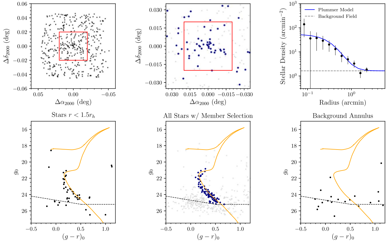
Figure 4. Diagnostic plots for DELVE J1448+1728 (DELVE 5) based on the GMOS-N data. Refer to Figure 3 for a detailed description of each panel. We highlight the unusual morphology of this system, which may suggest that it is not in dynamical equilibrium.
