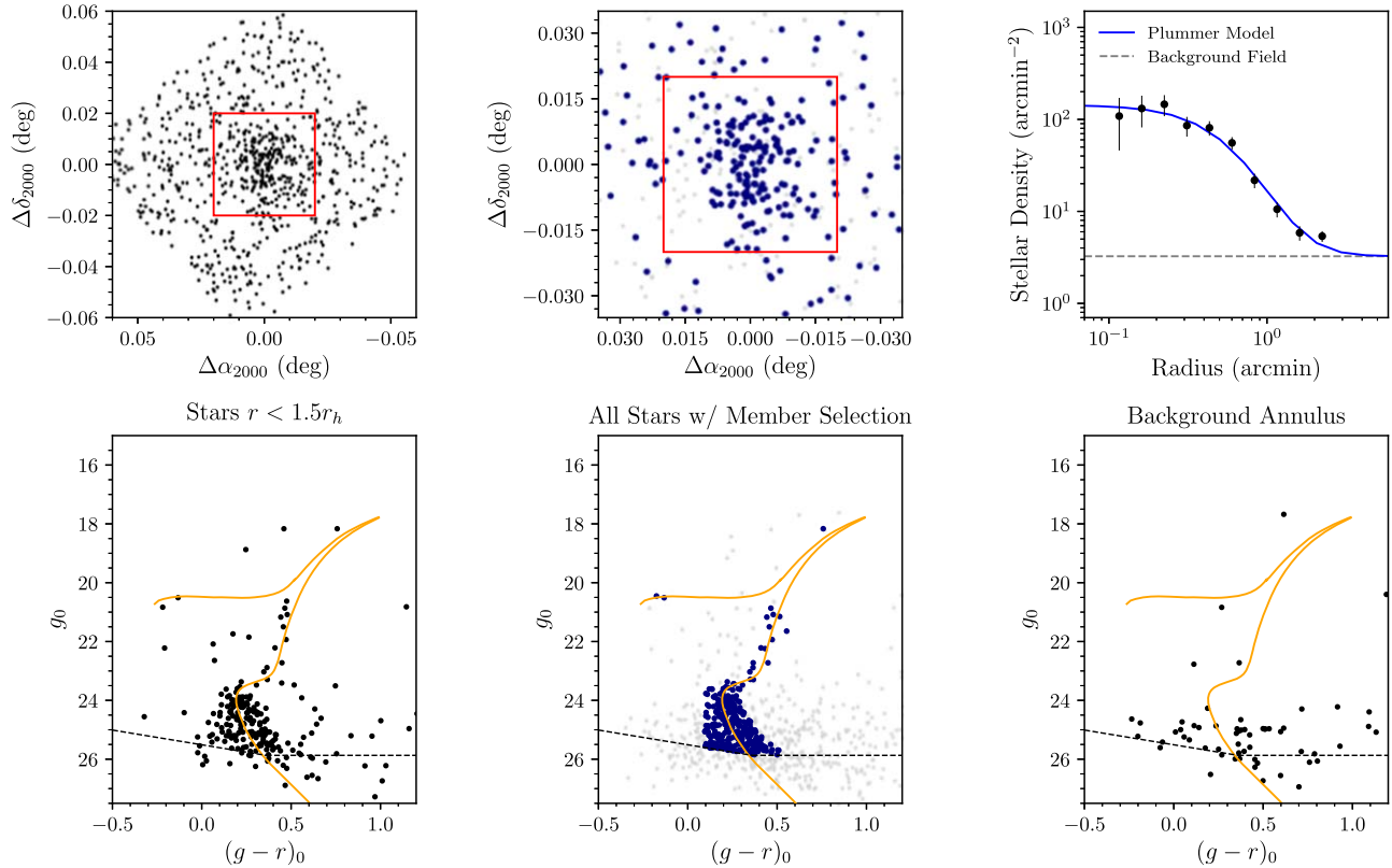
Figure 6. Diagnostic plots for DELVE J1415+3254 (Boötes V) based on the GMOS-N data. Refer to Figure 3 for a detailed description of each panel. We note that one candidate blue horizontal branch member star falls just outside our isochrone selection.
