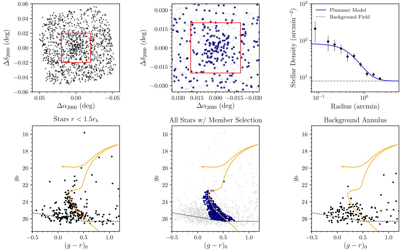
Figure 5. Diagnostic plots for DELVE J1500+0554 (Virgo II) based on the GMOS-N data. Refer to Figure 3 for a detailed description of each panel.
