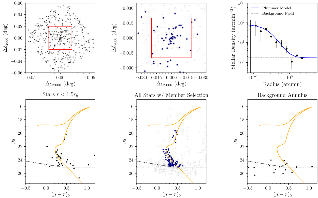
Figure 3. Diagnostic plots for DELVE J1523+2723 (DELVE 4), based on the GMOS-N data. (Top left) Spatial distribution of all stars in the full GMOS-N FOV; only our quality cut based on \chi and sharp has been applied. (Top center) A zoomed-in version of the top left panel, now including only stars above the magnitude limit reported in Table 1. Stars with colors consistent with the isochrone to within 0.07 mag, accounting for photometric errors, are colored in blue and are presumed to be members. (Top right) Radial profile of isochrone-filtered stars centered on DELVE J1523+2723, again including only stars above the magnitude limit. The best-fit azimuthally averaged Plummer model is shown as a solid blue curve, and the background field surface density is depicted as a black dashed line. (Bottom left) Color-magnitude diagram of stars within a circular selection of 1.5r_h centered on DELVE J1523+2723. The best-fit PARSEC isochrone is shown as a solid orange curve. The black dashed line denotes the magnitude limit used for our structural fit. (Bottom center) Color-magnitude diagram of stars within the GMOS-N FOV, with stars identified as candidate members colored as in the top-center panel. Stars identified as foreground based on their Gaia parallaxes and/or proper motions are excluded from this member selection, and are shown in gray. (Bottom right) Color-magnitude diagram for sources in a background annulus with inner radius of \sim 2' 4'' . This annulus nearly traces the perimeter of the GMOS-N FOV, and is equal in area to the selection used in the bottom-left panel.
