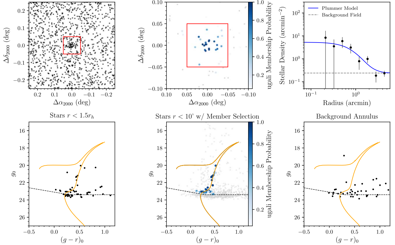
Figure 7. Diagnostic plots for DELVE J1057+2852 (Leo Minor I) based on the DECam data. Refer to Figure 2 for a detailed description of each panel. Although the total number of stars above the magnitude limit is relatively small, the radial stellar density profile appears accurately represented by the best-fit Plummer model.
