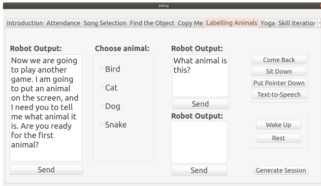
Fig. 2: Customized GUI.
