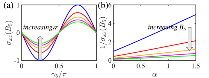
FIG. 5. Planar Hall conductivity for a minimal model of untilted TR broken WSM in the absence of any magnetic field. (a) Variation with respect to the angle \gamma_5 . Increasing \alpha reduces the conductivity, as expected. (b) PHC behaves as the inverse of scattering strength. Since \sigma_{xz}(B_5 = 0) = 0 , we have normalized \sigma_{xz} appropriately in both the plots. In creasing B_5 field increases the conductivity.
