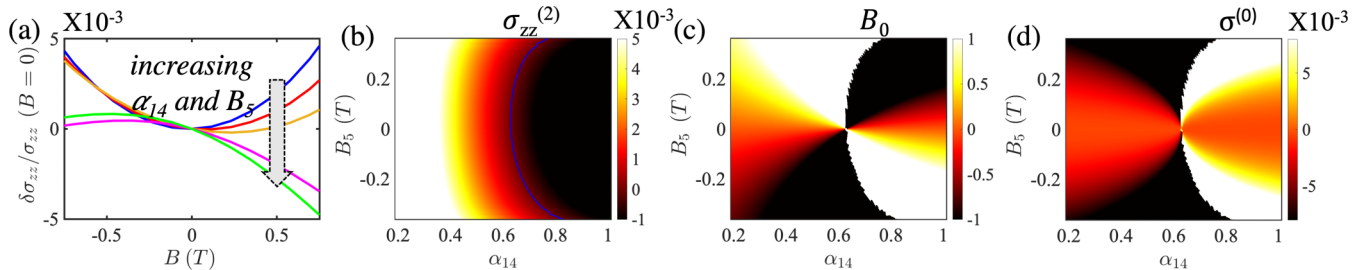
FIG. 18. (a) LMC for inversion asymmetric Weyl semimetal. As we move from the blue to the green curve, we simultaneously increase B_5 as well as \alpha_{14} . Both weak and strong sign-reversal are exhibited. The plots (b), (c), and (d) plot the parameters \delta\sigma_{zz}^{(2)} , B_0 , and \sigma^{(0)} for fixed \alpha_{12} and t_z \neq 0 . The blue contour in plot (b) separates the phases where \sigma_{zz}^{(2)} changes sign. Again, we see signatures of both weak and strong sign-reversal. The tilt parameter is fixed to t_z/v_F = -0.1 .
