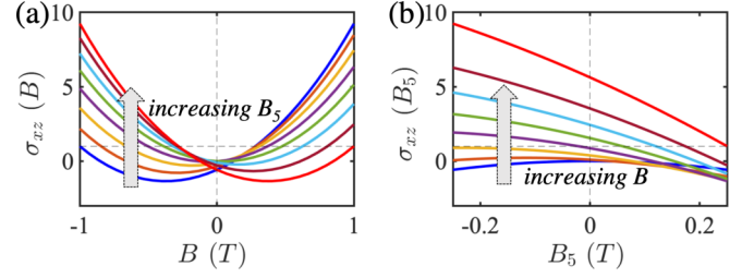
FIG. 8. Planar Hall conductance for a minimal model of untitled WSM. (a) As a function of the external B field. As we go from blue to red curve, we increase B_5 from -0.25 to +0.25 T. (b) As a function of the B_5 field. As we go from blue to red curve, we increase B from 0 to 1 T. All the plots are appropriately normalized. We chose \gamma = \gamma_5 = 0.45\pi , and \alpha = 0.5 .
