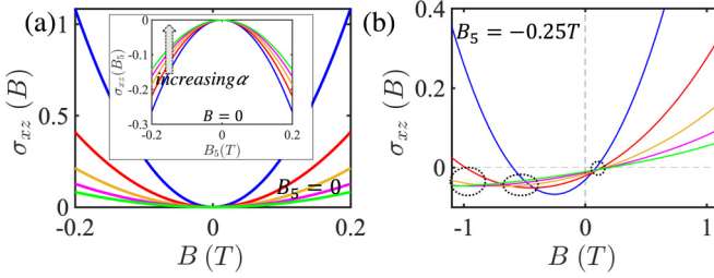
FIG. 6. Planar Hall conductivity for a minimal model of untitled TR broken WSM. (a) PHC as a function of external magnetic field B and no strain-induced field ( B_5 = 0 ) is compared with the inset where PHC has been plotted as a function of B_5 with no external field ( B = 0 ). The angle \gamma was chosen to be equal to \gamma_5 . Strain opposes the planar Hall effect albeit with different magnitude. (b) PHC in the presence of both magnetic field and strain. The chiral gauge field causes weak sign reversal. The dotted ellipses highlight regions that show an anomalous behavior with respect to intervalley scattering strength. The width of lines is reduced for better visibility. In all the curves, as we go from blue to green, we increase \alpha . All the plots are appropriately normalized.
