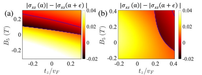
FIG. 14. Change in the magnitude of the planar Hall conductivity [\sigma_{xz}(\alpha) - |\sigma_{xz}(\alpha + \epsilon)|] for a tilted TR broken WSM [Eq. (5)] on infinitesimally increasing in the scattering strength (by \epsilon ). (a) The Weyl cones are tilted in opposite direction. (b) The Weyl cones are tilted in the same direction. In the region enclosed within blue contours, we find anomalous behavior of conductivity with the scattering strength, i.e., the magnitude of the conductivity increases on the increase of scattering strength. We choose \alpha = 0.5 and \epsilon = 0.01 .
