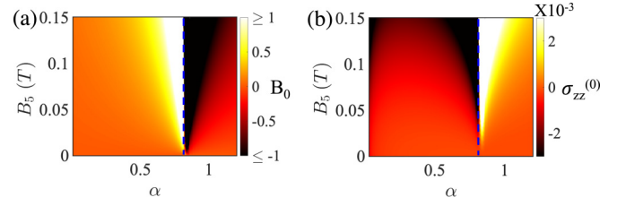
FIG. 3. (a) The vertex of the parabola B_0 , and (b) conductivity at B_0 for a minimal model of untitled TR broken WSM [Eq. (2)]. Around the blue dashed contour ( \alpha = \alpha_c ) we see strong sign reversal. The parameters B_0 and \sigma_{zz}^{(0)} show a striking change of sign as we move across the \alpha_c contour.
