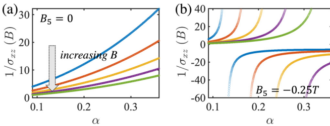
FIG. 7. Planar Hall conductance for a minimal model of untitled WSM as a function of intervalley scattering strength. (a) In absence of B_5 field. (b) In presence of B_5 field. In all the curves, as we go from blue to green, we increase B . All the plots are appropriately normalized.
