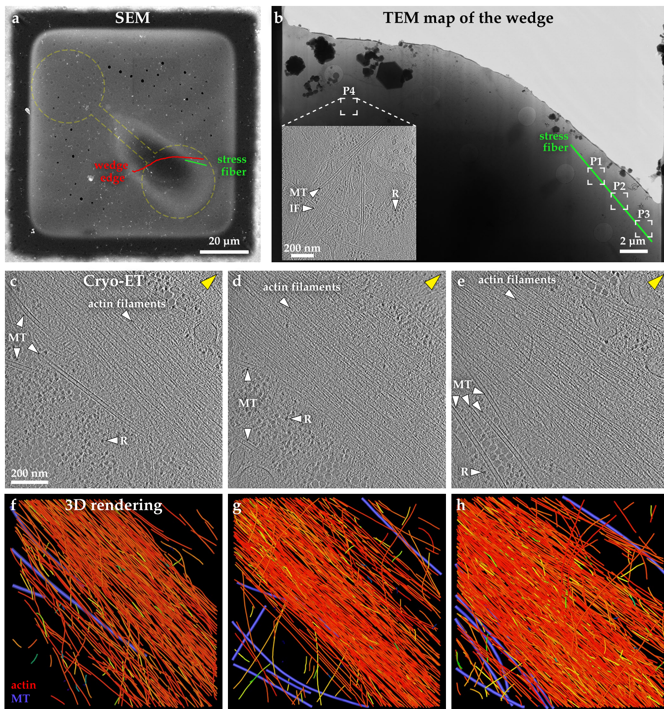
Extended Data Fig. 5 | Actin filament organisation in 3D within and near the stress fiber. a. Cryo-Scanning Electron Microscopy of a vitrified RPE1 cell adhered and spreading on a dumbbell-shape micropattern. Red line indicates the putative position of the edge of the wedge produced by cryo-FIB milling. The green line indicates the position of the stress fiber imaged by cryo-ET. The yellow dashed line represents the dumbbell shape pattern size and position. b. Cryo-TEM of the wedge of the RPE cell shown in (a) , displaying the positions (P1-P4) for cryo-ET. Inset: 6.8 nm thick tomographic slice of the P4 region. Microtubules (MTs); ribosomes (R); intermediate filaments (IF). c-e. Cellular cryo-ET. Tomographic slices (6.8 nm thickness) of three positions - P1, P2 and P3 - in (b) , respectively, along the same stress fiber. The three tomograms start at the basal membrane and extend the thickness of the tomograms towards the apical membrane. The distance between consecutive tomographed positions is ~ 2.5 µm (center-to-center of the tomograms), covering a total distance of ~7 µm. N=2 experiments. f-h. 3D rendering of the actin filament network and microtubules (purple) from (c-e) , respectively. Blue-to-red color map of actin filaments represent the angular distribution (ranging from 0° to 90°) relative to the z-plane of the tomogram. Most actin filaments are positioned parallel to the basal membrane. See related Video 5.
