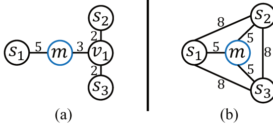
Figure 2: f_{MKSP} examples.
