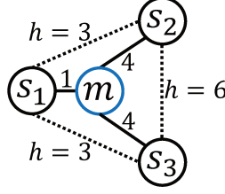
Figure 4: Clique heuristic example.
