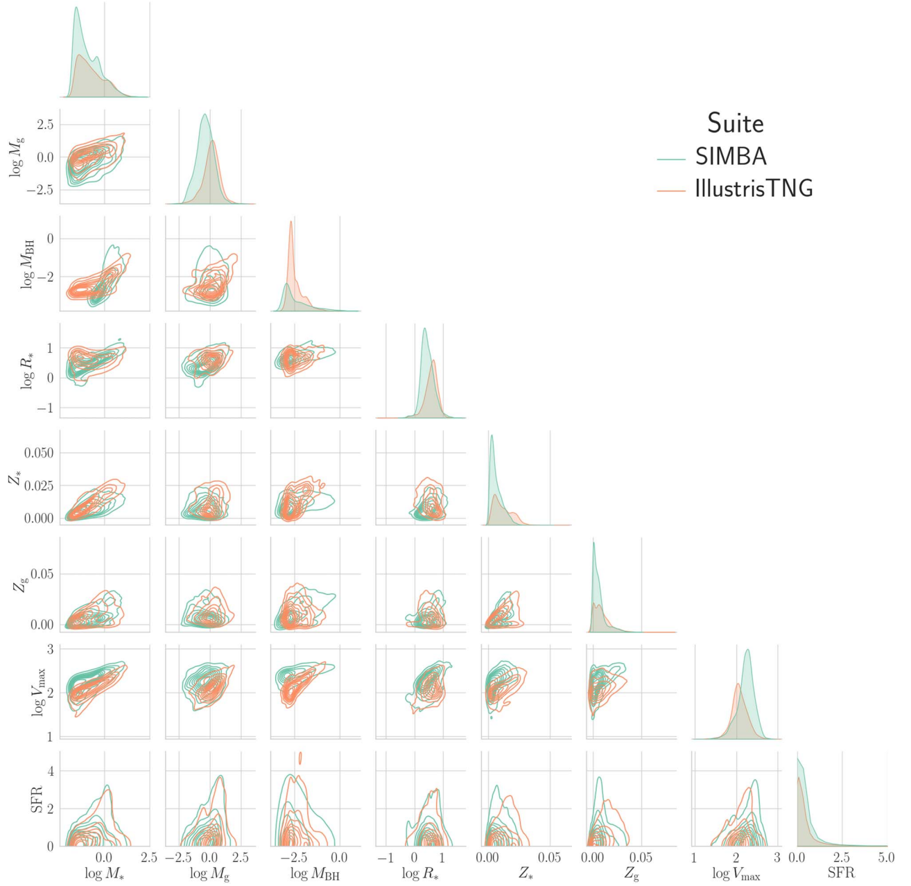
Figure 2. In this plot, we illustrate the similarities and differences between the IllustrisTNG and SIMBA suites considering eight different properties of the subhalos: (1) stellar mass, M_* , (2) gas mass, M_g , (3) black hole mass, M_{BH} , (4) stellar half-mass-radius, R_* , (5) stellar metallicity, Z_* , (6) gas metallicity, Z_g , (7) maximum circular velocity, V_{max} , and (8) star formation rate, SFR. We show the 1D and 2D distribution of these properties for all galaxies in the LH sets of the IllustrisTNG (orange) and SIMBA (green) suites. Masses are in units of 10^{10}/(M_\odot h^{-1}) , R_* in kiloparsecs per hour, V_{max} in kilometers per second, and SFR in M_\odot \text{ yr}^{-1} .
