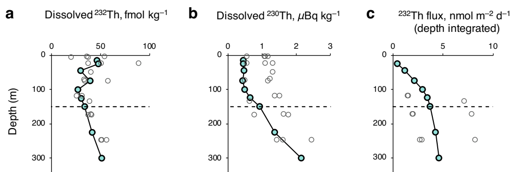
Fig. 3. Thorium isotope distributions at Station ALOHA. Profiles of ^{232}\text{Th} ( a ), ^{230}\text{Th} ( b ), and the inferred flux of ^{232}\text{Th} ( c ), derived as per Hayes et al. (2013). Observations from June 2019 are plotted in cyan. Gray circles indicate past measurements at Station ALOHA reported by Hayes et al. (2015). The dashed line at 150 m highlights the integration depth used for mass balance calculations, see “Results” section.
