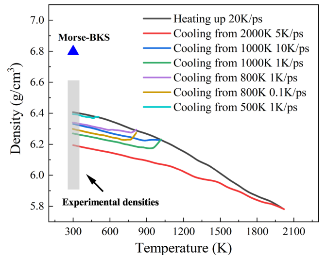
FIG. 5. Temperature vs atomic density of amorphous models during simulated annealing. The blue triangle represents models from Morse-BKS potentials. The gray region is the experiment densities.
