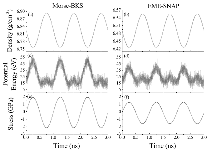
FIG. 6. Mechanical spectroscopy simulations of 50% \text{ZrO}_2 -doped \text{Ta}_2\text{O}_5 . The frequency of the strain is 1 \times 10^9 Hz at 300 K. (a), (c), and (e) are from models with the Morse-BKS potential, and (b), (d), and (f) are from models with EME-SNAP.
