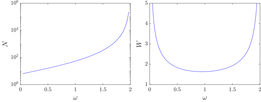
FIG. 1. Dependence of the norm and the width of the solitary wave with respect to its frequency for the relevant family of solutions.
