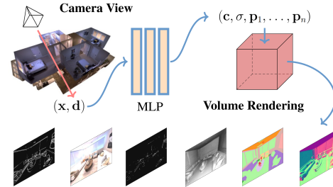
Figure 1: We represent the scene as an implicit function and develop a versatile neural scene representation, SS-NeRF, that is able to not only render images from novel viewpoints, but also render various scene properties (e.g., appearance, geometry, and semantics) paired with the synthesized images, under a unified framework.
