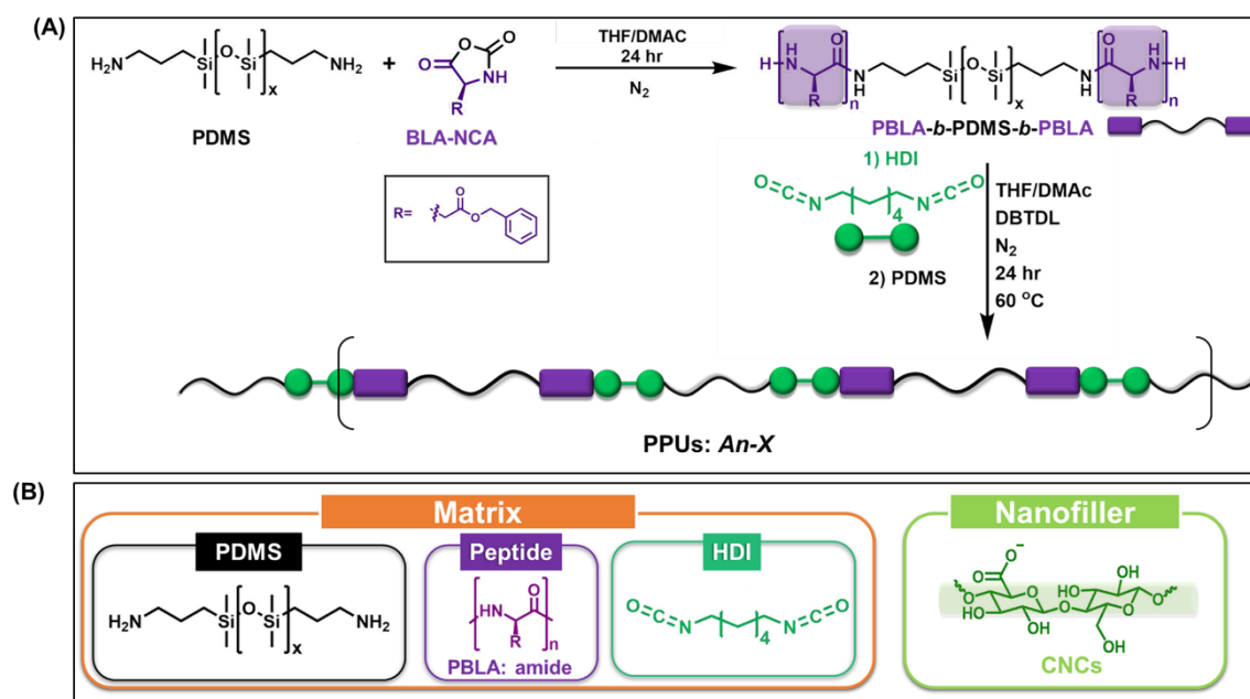
Figure 1. (A) Synthetic scheme of PPU (matrix) and (B) building blocks (i.e., matrix and nanofiller) used to design a new type of PPU/CNC nanocomposites.
