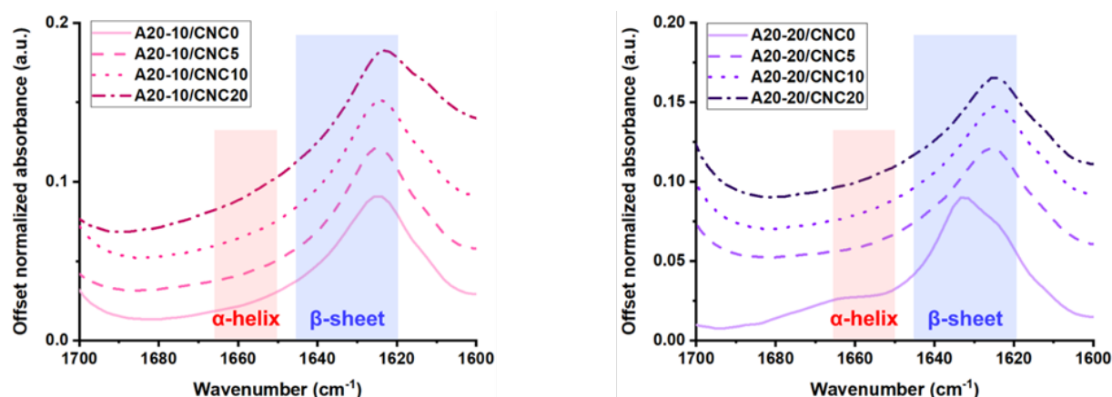
Figure 2. ATR-FTIR spectra of PPU/CNC nanocomposites as a function of the CNC weight fraction. Peptide secondary structure was identified based on the second derivative in the amide I stretching region (1700–1600 \text{cm}^{-1} ). CNC incorporation into PPUs leads to variations in secondary conformation, disrupting \alpha -helical ordering but promoting intermolecular hydrogen bonding. This finding provides evidence of preferential interactions between the PBLA blocks and CNCs.
