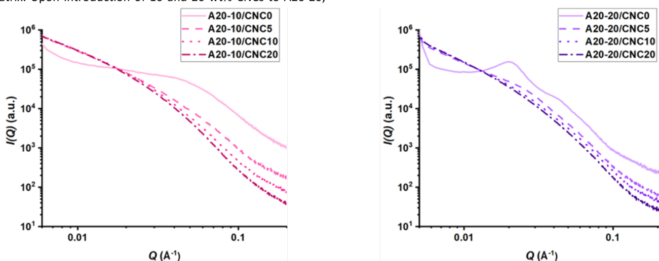
Figure 4. 1D-SAXS profiles of the PPU/CNC nanocomposites with varying PBLA and CNC content collected at room temperature for 30 minutes. The neat PPU matrices ( i.e. , A20-10/CNC0 and A20-20/CNC0) exhibit a defined scattering peak, whereas the addition of CNC to the matrices results in a reduction or loss of the distinct peak. These results indicate that the introduction of CNCs into PPU matrices modulates long-range ordering and structural hierarchy.
