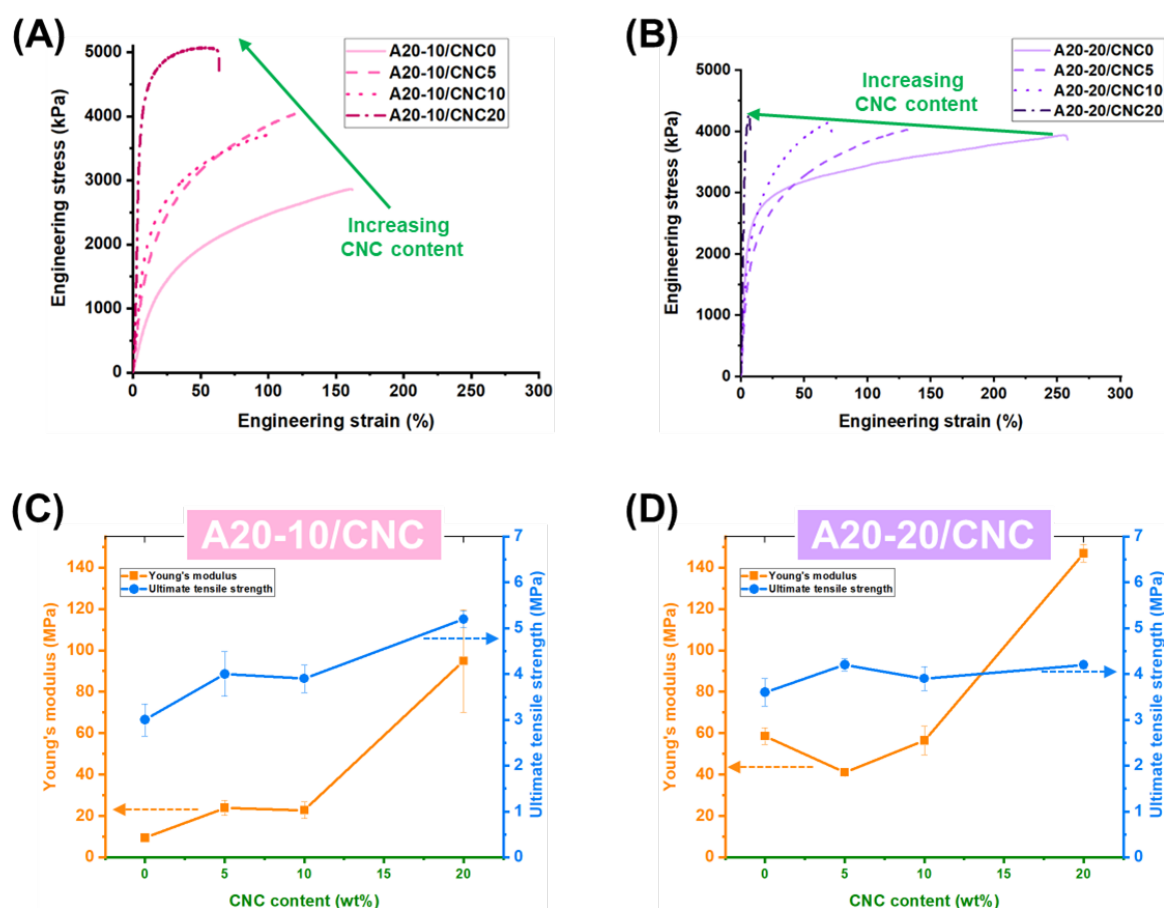
Figure 6. Representative stress-strain curves of (A) A20-10/CNC and (B) A20-20/CNC measured via ZwickRoell mechanical testing machine (with a 100 N load cell) in tension mode at room temperature under a constant strain rate of 100% of the initial gauge length/min (At least three samples with dimensions of \sim 3 \times 15 mm were tested for each material.). Young's modulus and ultimate tensile strength of (C) A20-10/CNC and (D) A20-20/CNC obtained by averaging the results of three samples, which highlight that Young's modulus is highly influenced by the PBLA content and CNC weight fraction compared with tensile strength. Young's modulus of A20-10/CNC nanocomposites increases from 9 MPa to 95 MPa with increasing CNC weight fractions from 0 wt% to 20 wt%, which contrasts with A20-20/CNC nanocomposites. Particularly, A20-20/CNC5 (41 MPa) exhibits a lower Young's modulus compared to neat A20-20 (59 MPa). Increasing the amount of CNCs in A20-20 to 20 wt% enables obtaining a higher Young's modulus up to 147 MPa. This tensile behavior reveals that a balance of peptidic ordering and PBLA-CNC interactions dictates the mechanical response of PPU/CNC nanocomposites.
