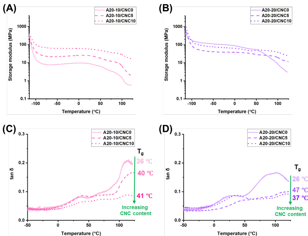
Figure 5. DMA curves of neat PPU and CNC-reinforced PPU with varying CNC weight fractions, recorded in oscillatory film tension mode at a heating rate of 5 °C/min and a frequency of 1 Hz. Top: storage modulus; Bottom: \tan \delta (the ratio of loss modulus over storage modulus) with summarized PBLA glass transition temperatures ( T_g – peak in \tan \delta ). (A) and (C) A20-10/CNC series; (B) and (D) A20-20/CNC series. Increasing CNC content in A20-10 yields a higher storage modulus, whereas incorporating CNC into A20-20 reduces a storage modulus. In both A20-10 and A20-20, T_g increases when CNCs are added, suggesting that the chain mobility is restricted. These data support that the peptide content and hierarchical structures of PPU have a significant impact on the thermomechanical properties of PPU/CNC nanocomposites. This finding demonstrates the importance of not only matrix-filler interactions but also the hierarchy of matrix material in tuning mechanical performance.
