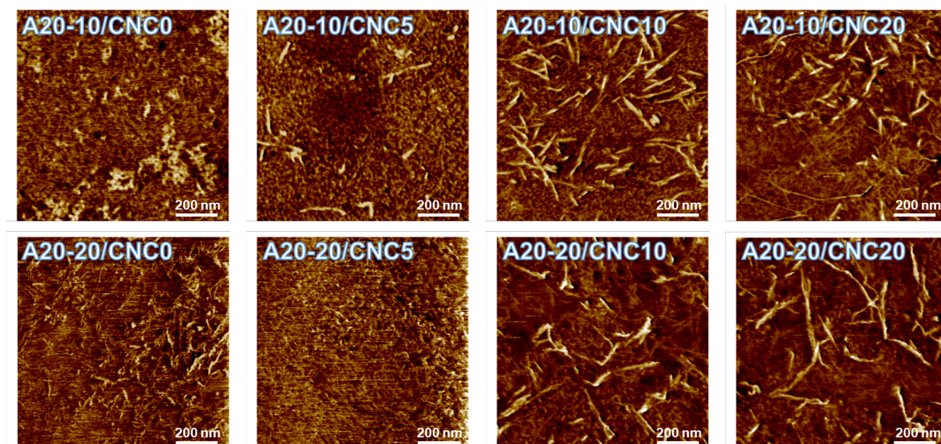
Figure 3. Tapping-mode AFM phase images of the A20-10/CNC and A20-20/CNC nanocomposites (image size: 1 \times 1 \mu\text{m} , scan rate: 1 Hz). These images show the rod-like structures of A20-10 and A20-20 disappear upon CNC loading in PPU, indicating that a change of hydrogen bonding arrangements from PBLA-PBLA to PBLA-CNC results in phase separation behavior.
