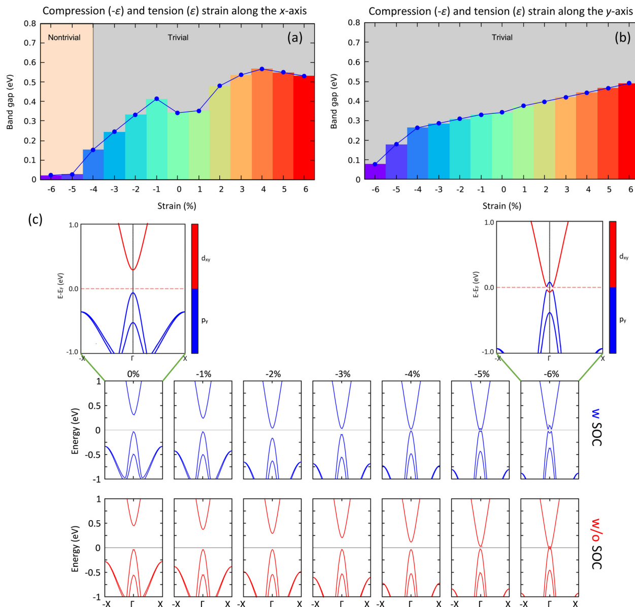
Fig. 5 The variation of the bandgap at the \Gamma point of the TiNI monolayer under uniaxial strain ( -6 \leq \varepsilon_{x/y} \leq 6\% ) along the x-axis (a) and y-axis (b) in the presence of SOC within the HSE06 approach. (c) Band structures of the TiNI monolayer under the external uniaxial compression strains along the x-axis without and with SOC. To correct the electronic structure states, we employed the HSE06 approach. When the SOC effect is not considered, the energy bandgap gradually decreases with decreasing lattice constant ( a_0 ), and when it reaches -6\% , the bandgap closes. In this case, like the PBE-GGA approach, the band structure shows a semimetallic character with the Dirac semimetal points slightly away from the \Gamma point along the -X-\Gamma-X direction. Considering the SOC simultaneously, a nontrivial bandgap opens. The I-p_y and Ti-d_{xy} orbital-resolved band dispersions within the HSE06 approach of TiNI monolayer near E_F with SOC for 0% and -6\% are calculated.
