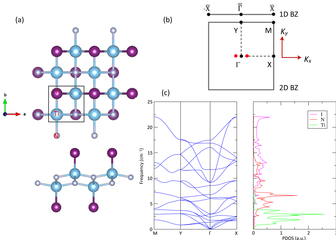
Fig. 1 (a) Top and side views of the crystal structure of the TiNI monolayer; the unit cell is indicated with a solid black square. (b) 2D and 1D BZ with specific symmetry points. The red dots represent Dirac points located at P = (k_x = \pm 0.045, k_y = 0.0) \text{ \AA}^{-1} in the 2D BZ. (c) Phonon dispersion and PDOS of the TiNI monolayer at its equilibrium lattice parameters. All the branches have positive frequencies without any imaginary phonon modes in the entire BZ, evidencing the dynamic stability of this monolayer.
