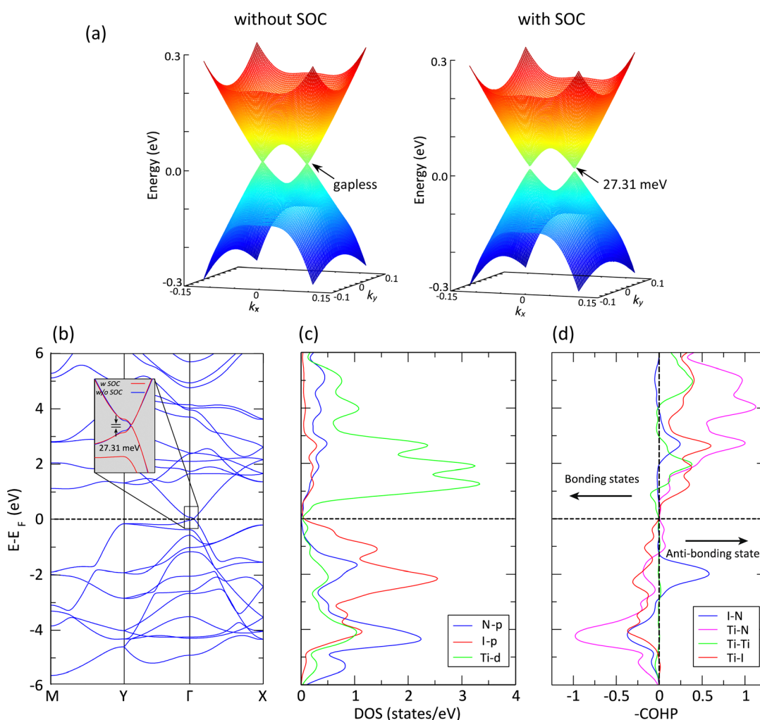
Fig. 2 (a) The 3D electronic band structures of TiNI monolayer using PBE-GGA scheme in the presence and absence of SOC. Without including SOC, TiNI monolayer is gapless. The inclusion of SOC opens up a bandgap of 27.31 meV, which is due to the presence of the heavy element iodine. (b) The calculated band structures without SOC at high symmetry point. The inset shows the band structure around the \Gamma point with (red color) and without (blue color) SOC. (c) Electron partial density of states (DOS) projected onto different atoms and orbitals of the TiNI monolayer. (d) The crystal orbital Hamiltonian populations (COHP) diagram. The negative and positive values of COHP indicate anti-bonding and bonding states, respectively.
