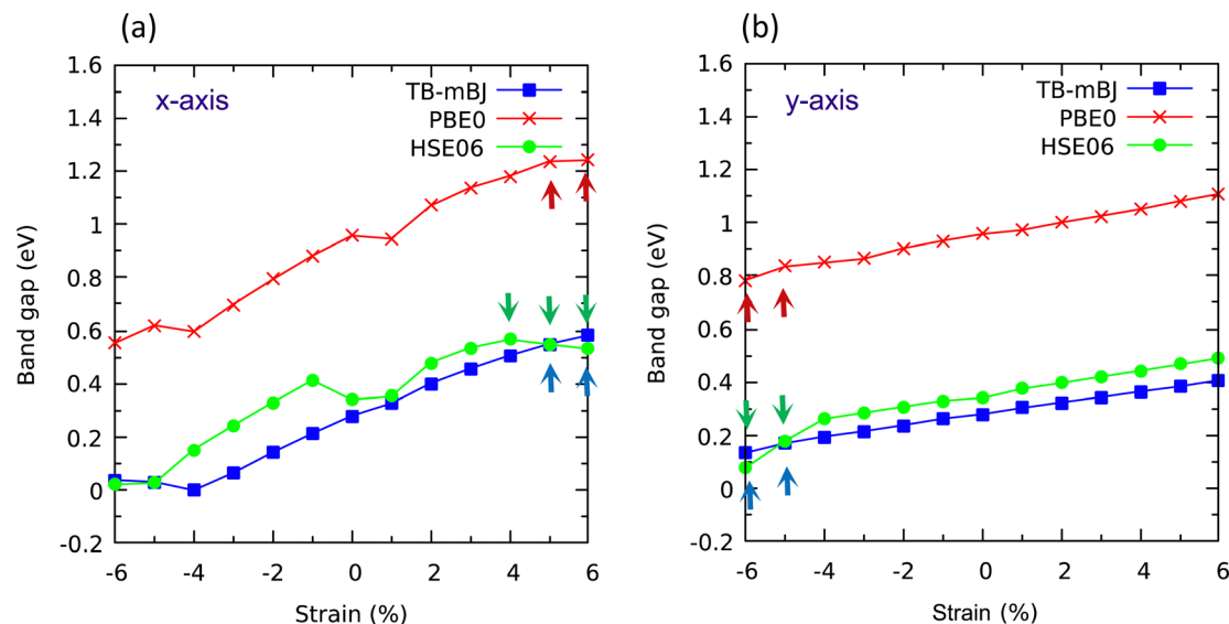
Fig. 6 The variation of the bandgap of the TiNI monolayer under uniaxial strain (−6% to 6%) along the (a) x-axis and (b) y-axis. Three approaches (HSE06, PBE0, and TB-mBJ) were used to analyze the changes in the bandgap. Colored arrows indicate indirect band gaps ( \Gamma \rightarrow X ).
