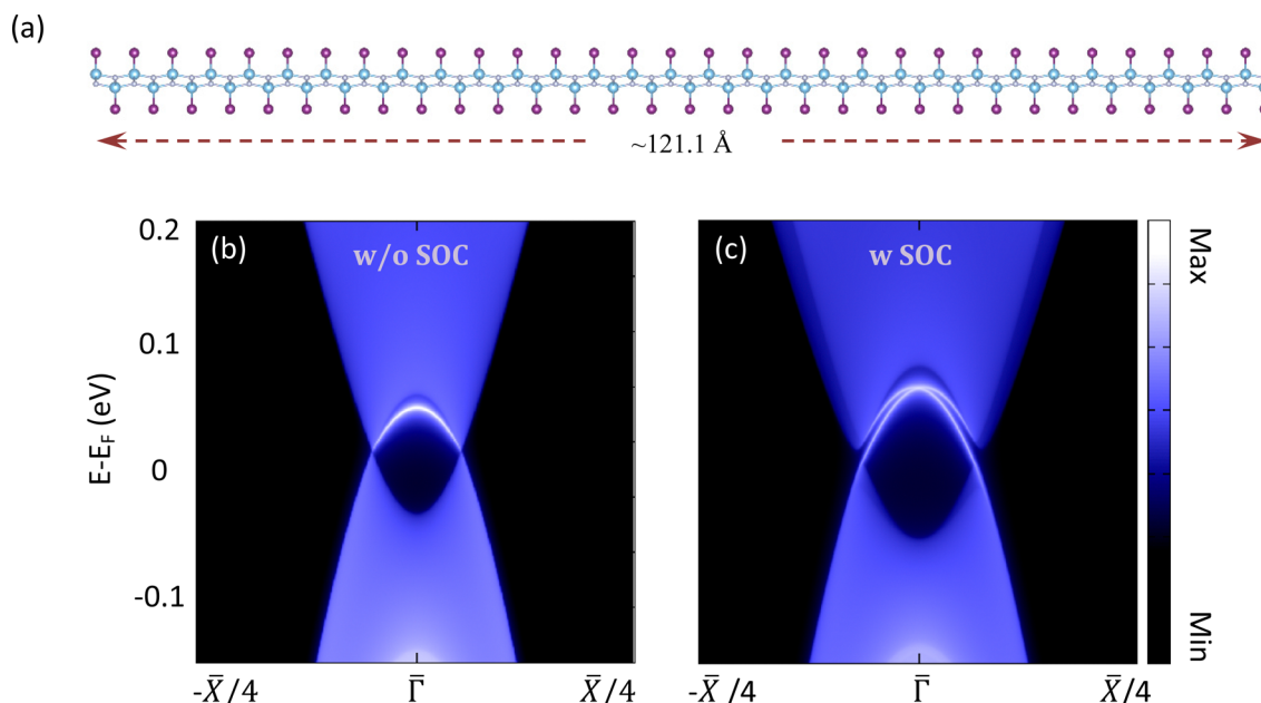
Fig. 4 (a) The nanoribbon width is set to 121.1 Å to avoid the interaction between the edges. The local density of states without (b) and with (c) SOC inclusion. In the absence of the SOC, there are two topological edge states (two branches of the edge states overlap) connecting two 2D Dirac semimetals along the high symmetry line -\bar{X}-\bar{\Gamma}-\bar{X} . With the inclusion of the SOC, the two branches of the topological edge states split due to the energy gap opening, connecting the valence and conduction bands.
