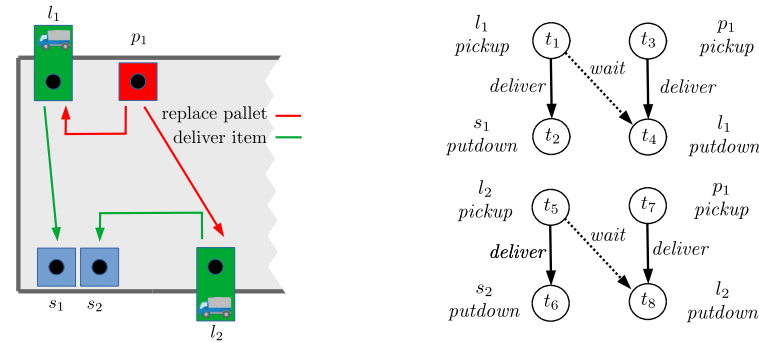
Figure 2. Item deliveries from l_1 to s_1 and from l_2 to s_2 . Their corresponding replacement empty pallet deliveries are from p_1 to l_1 and l_2 , respectively.
