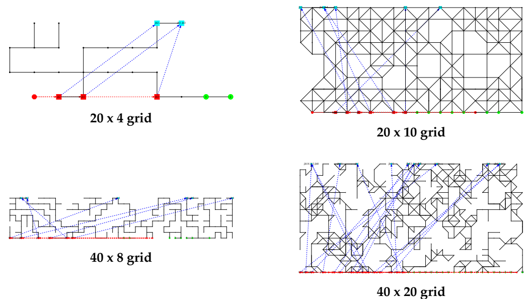
Figure 5. Example synthesized warehouse graphs. Circular green vertices indicate robot home locations. Square red vertices indicate full pallet pickup locations with a dotted blue arrow pointing to the corresponding storage location. Octagonal red vertices indicate empty pallet pickup locations with a dotted red arrow pointing to the delivery location for the corresponding empty pallet.
