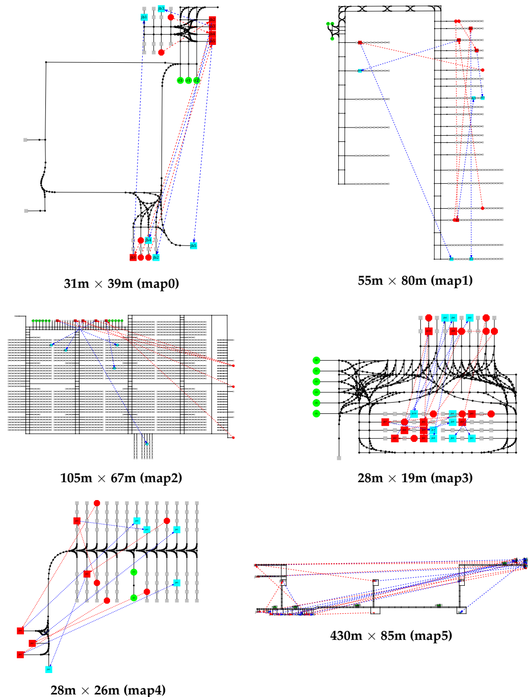
Figure 6. Example instances for the real-world warehouse graph. Circular green vertices indicate robot home locations. Square red vertices indicate full pallet pickup locations with a dotted blue arrow pointing to the corresponding storage location. Octagonal red vertices indicate empty pallet pickup locations with a dotted red arrow pointing to the delivery location for the corresponding empty pallet.
