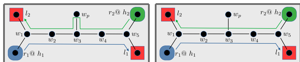
Figure 3. A simple example showing the limitation of the path encoding against the step-based encoding; robot r_1 located at vertex h_1 needs to travel to l_1 , while robot r_2 at h_2 needs to travel to l_2 . For a uniform edge weight of 10 s the walk encoding (left) can achieve the optimal makespan of 90 s while the best path encoding plan (right) requires 120 s.
