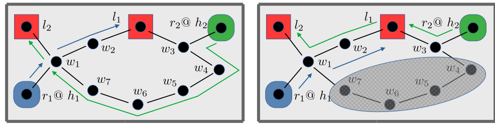
Figure 4. A simple example showing the limitation of the corridor-based routing; robot r_1 located at vertex h_1 needs to travel to l_1 , while robot r_2 at h_2 needs to travel to l_2 . For a uniform edge weight of 10 s the corridor-free encoding ( left ) can achieve the optimal makespan of 70 s by sending r_2 along a non-shortest path route, while the corridor-based encoding ( right ) rules out vertices w_4, \dots, w_7 from the corridor and requires 80 s.
