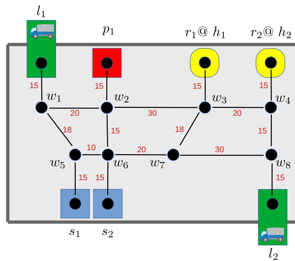
Figure 1. A graph representing a simple warehouse with loading bay vertices l_1 and l_2 , an empty pallet area p_1 , storage vertices s_1, s_2 , waypoint vertices w_1, \dots, w_8 , and home vertices h_1, h_2 for robots r_1, r_2 , respectively. Edge labels represent the minimal travel times between vertices (in seconds).
