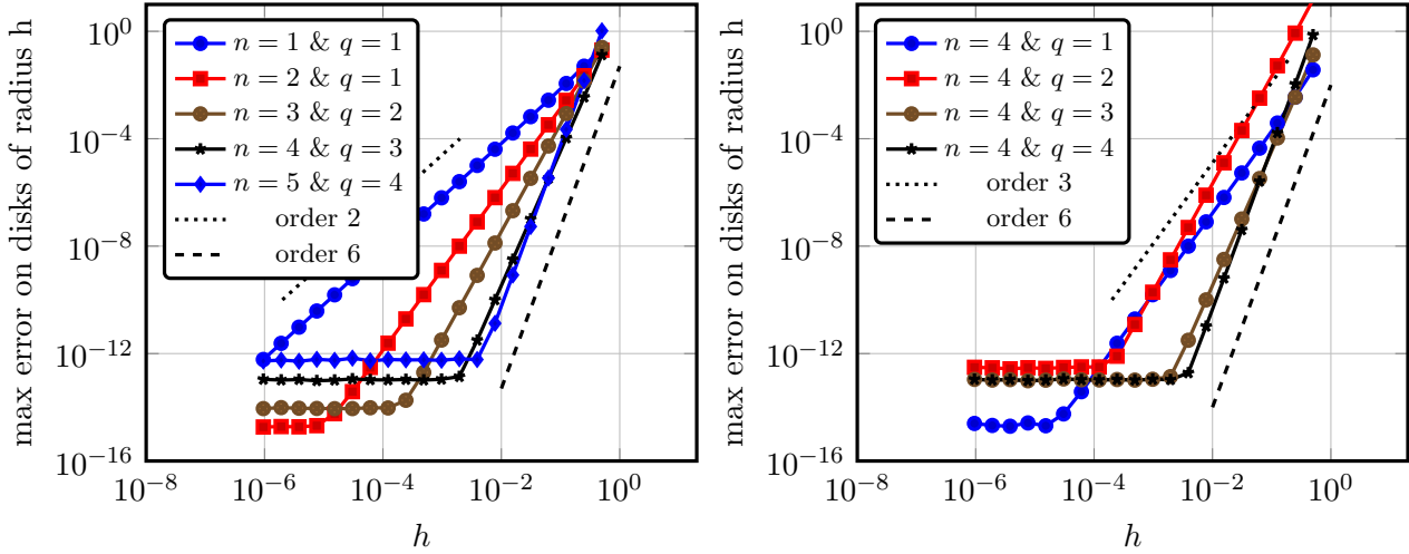
Figure 8: GPW approximation of u_{cs} by u_a \in \mathbb{V}_{\alpha,p,q}^0 with p = 2n + 1 . We represent the L^\infty error \max_{(x_0,y_0) \in \Omega} \|u_{cs} - u_a\|_{L^\infty(\{(x,y) \in \mathbb{R}^2, |(x,y) - (x_0,y_0)| < h\})} , for 50 random points (x_0, y_0) \in \Omega_{cs} . We compare results for parameters satisfying Theorem 1 hypotheses i.e. q = \max(1, n - 1) (Left panel), and for varying q with fixed n (Right panel).
