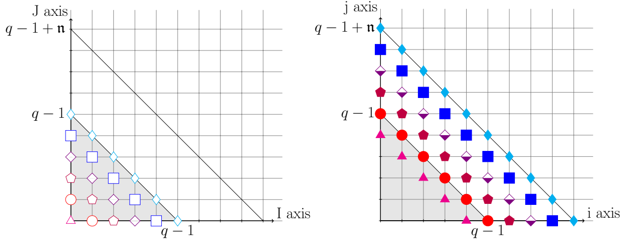
Figure 2: Representation of the indices of equations and unknowns from the initial nonlinear system (10) divided up into linear subsystems (21). For q = 6 and M = 4 , each shape of marker corresponds to one value of \mathfrak{L} : the indices (I, J) satisfying I + J = \mathfrak{L} correspond to the subsystem's equations (Left panel), while the indices (i, j) satisfying i + j = \mathfrak{L} + M correspond to the subsystem's unknowns (Right panel).
