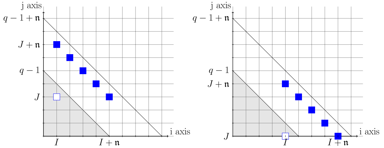
Figure 3: Representation of the indices of unknowns involved in two equations (I, J) of the subsystem (21). For q = 6 , for M = 4 , and \mathfrak{L} = 4 , each filled blue square marker corresponds in the (i, j) plane to an unknown \lambda_{ij} , involved in the (I, J) = (1, 3) equation (Left panel), or in the (I, J) = (4, 0) equation (Right panel).
