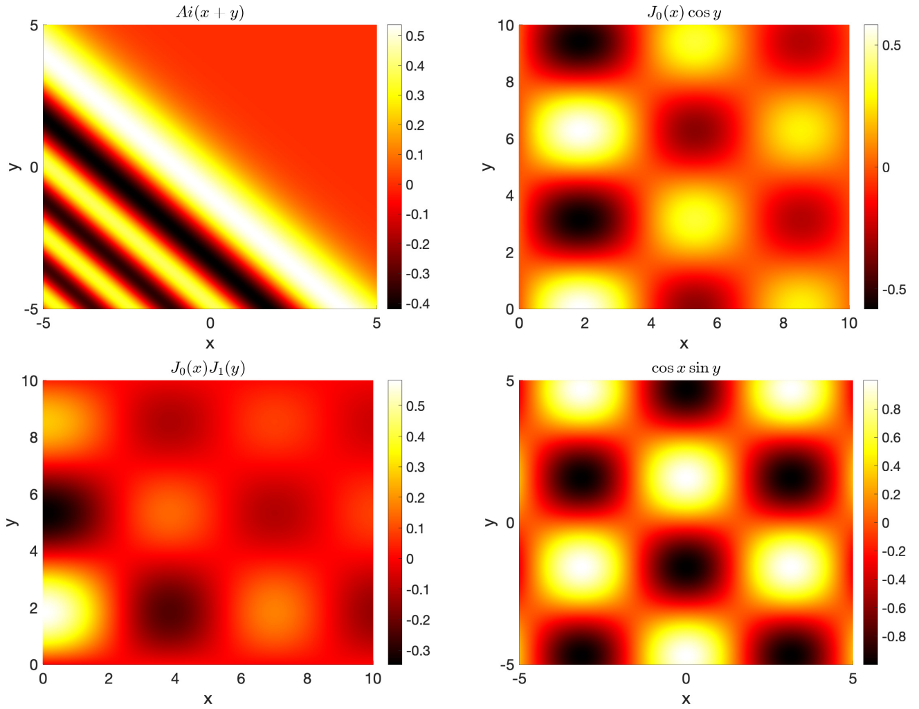
Figure 4: Exact solutions of the four test cases.
