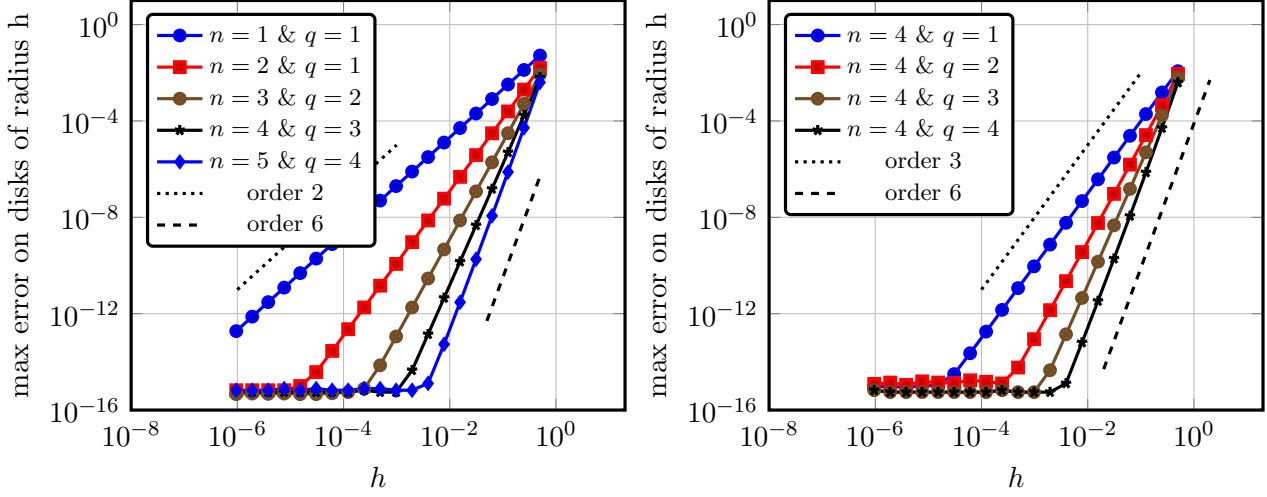
Figure 6: GPW approximation of u_{Jc} by u_a \in \mathbb{V}_{\alpha,p,q}^0 with p = 2n + 1 . We represent the L^\infty error \max_{(x_0,y_0) \in \Omega} \|u_{Jc} - u_a\|_{L^\infty(\{(x,y) \in \mathbb{R}^2, |(x,y) - (x_0,y_0)| < h\})} , for 50 random points (x_0, y_0) \in \Omega_{Jc} . We compare results for parameters satisfying Theorem 1 hypotheses i.e. q = \max(1, n - 1) (Left panel), and for varying q with fixed n (Right panel).
