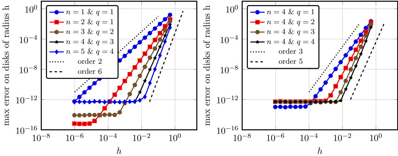
Figure 5: GPW approximation of u_{Ad} by u_a \in \mathbb{V}_{\alpha,p,q}^0 with p = 2n + 1 . We represent the L^\infty error \max_{(x_0,y_0) \in \Omega} \|u_{Ad} - u_a\|_{L^\infty(\{(x,y) \in \mathbb{R}^2, |(x,y) - (x_0,y_0)| < h\})} , for 50 random points (x_0, y_0) \in \Omega_{Ad} . We compare results for parameters satisfying Theorem 1 hypotheses i.e. q = \max(1, n - 1) (Left panel), and for varying q with fixed n (Right panel).
