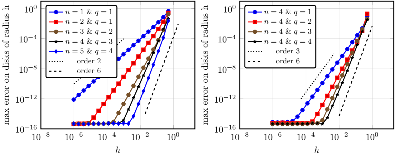
Figure 7: GPW approximation of u_{JJ} by u_a \in \mathbb{V}_{\alpha,p,q}^0 with p = 2n + 1 . We represent the L^\infty error \max_{(x_0,y_0) \in \Omega} \|u_{JJ} - u_a\|_{L^\infty(\{(x,y) \in \mathbb{R}^2, |(x,y) - (x_0,y_0)| < h\})} , for 50 random points (x_0, y_0) \in \Omega_{JJ} . We compare results for parameters satisfying Theorem 1 hypotheses i.e. q = \max(1, n - 1) (Left panel), and for varying q with fixed n (Right panel).
