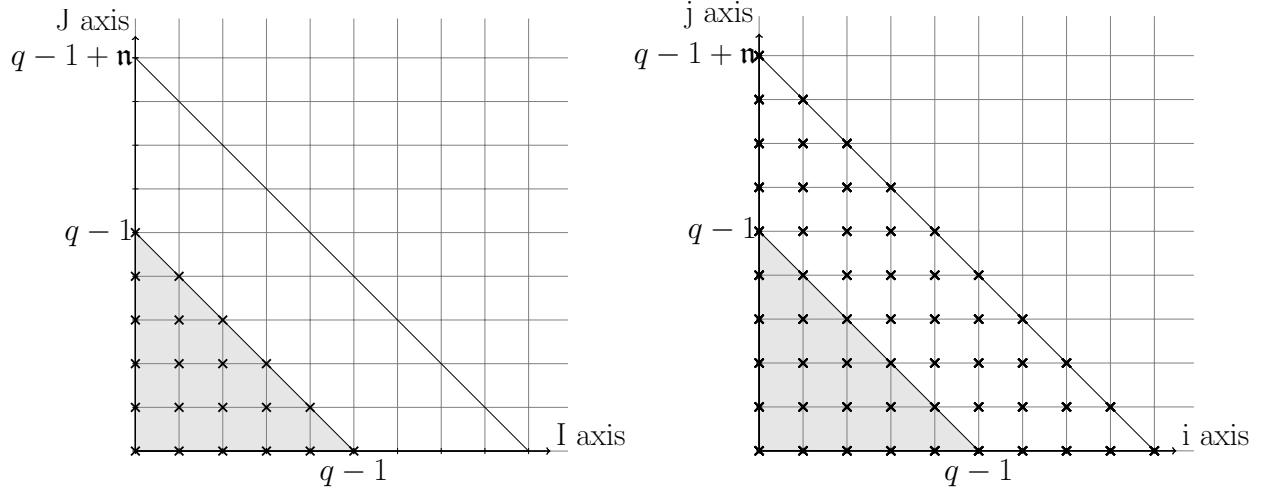
Figure 1: Representation of the indices involved in the nonlinear system (10), for q = 6 and n = 4 . Each cross in the (I, J) plane corresponds to the equation (I, J) in System (10) (Left panel), while each cross in the (i, j) plane corresponds to the unknown \lambda_{ij} (Right panel).
