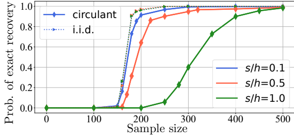
Figure 2: Probability of exact recovery of the matrix \Phi = \theta w^\top \in \mathbb{R}^{d \times h} from the noiseless measurement y = \langle Z, \Phi \rangle using low-rank recovery ( d = 10 and h = 100 ). We compare two types of design matrices: 1) Z with i.i.d. entries, and 2) circulant Z generated by an i.i.d. vector. Different instances, where w has different sparsity (quantified by s ), are considered. The experiment shows that: 1) the same amount of data is needed for all instances if Z has i.i.d. entries, but 2) the number of samples needed varies significantly when it comes to circulant Z . These observations indicate that for circulant measurements, the amount of data needed to recover a low-rank matrix may not simply depend on the rank, which is substantially different from i.i.d. measurements.
