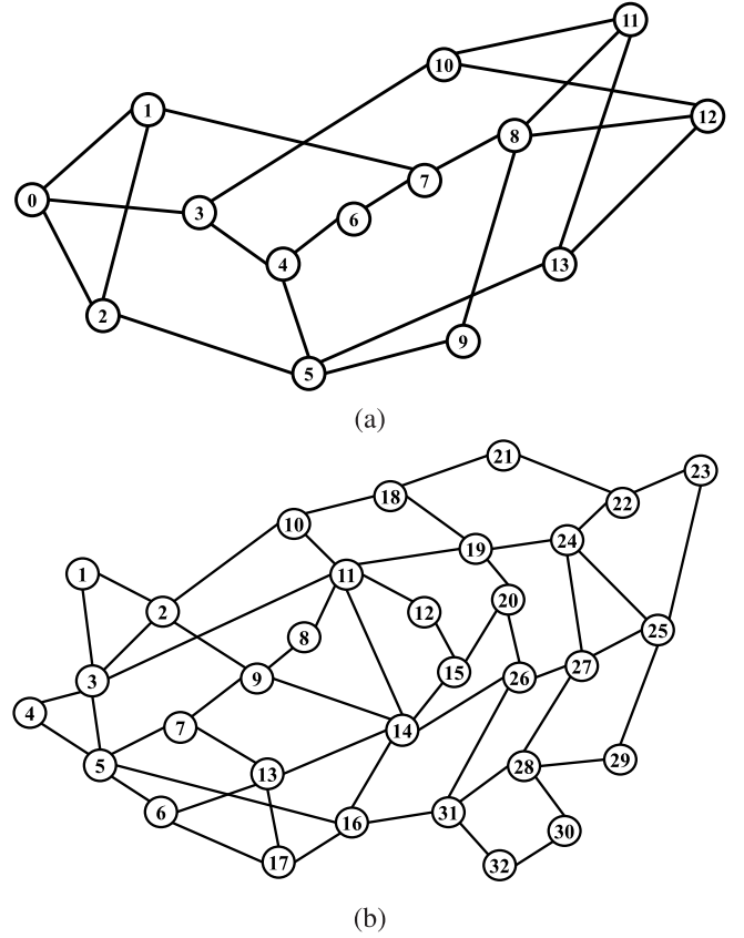
Fig. 4. Network topologies used in our study: (a) NSFNET, (b) GEANT2.
