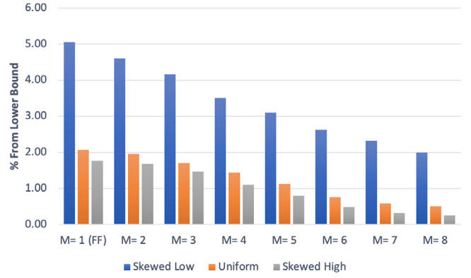
Fig. 6. PFF( M ) solution quality as % from LB, GEANT2.
