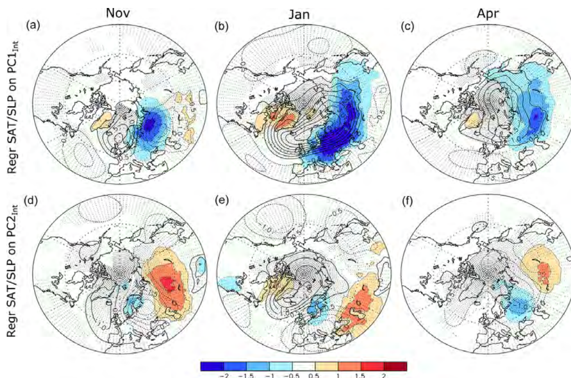
Figure 12. Regression of the (color shading) 2 m air temperature ( T_{2m} , °C) and (black contour, contour interval 0.5 hPa) SLP (hPa) on (a–c) PC1_{Int} and (d–f) PC2_{Int} for (left, a, d, and g) November, (center, b, e, and h) January, and (right, c, f, and i) April. All regressions are calculated at no lag (lag 0 months) and only use the T_{2m} and SLP anomalies associated with the internal atmosphere–land variability, after the removal of the corresponding multi-model mean. The regression shows the multi-model mean regression map, with dots indicating when the sign of SLP anomalies is consistent in at least seven models out of eight. The color shading is masked if the sign of T_{2m} is not consistent in at least seven models out of eight.
