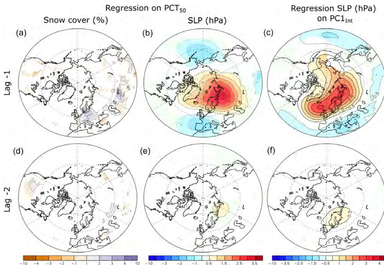
Figure 16. Regression of the (a,d) snow cover (%) and sea level pressure (SLP; b,e) anomalies (hPa) onto the January polar cap (north of 60° N) 50 hPa temperature anomalies in LMDZOR6. (c,f) Regression of the sea level pressure (SLP) anomalies (hPa) onto the first PC of the snow cover internal atmospheric variability, PC1 Int , in January and LMDZOR6. The lag indicated is negative and given in months, indicating that the polar cap 50 hPa geopotential height or the PC1 Int lags. The color shading is masked if the local statistical significance is above 5 %.
