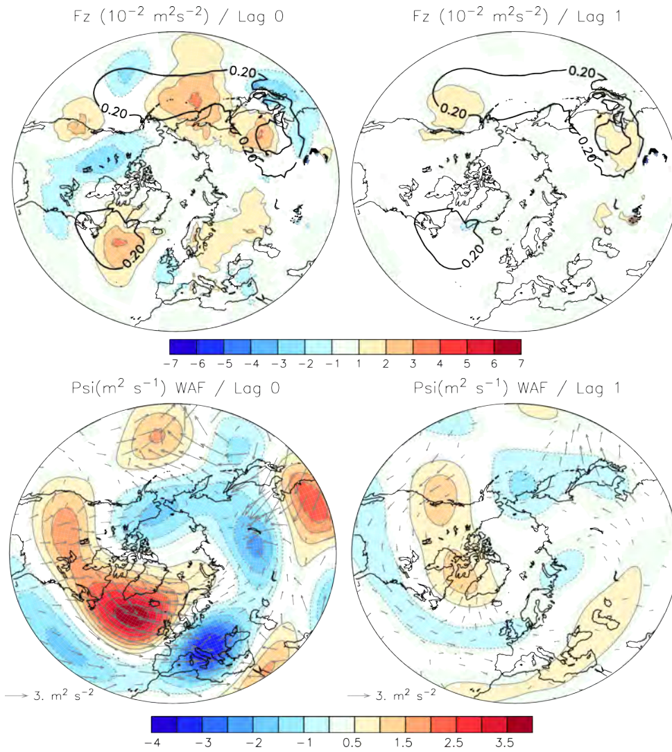
Figure S5: (Upper panels) Regression of the 500-hPa vertical component of the Plumb flux, in \text{m}^2 \text{ s}^{-2} , on January PC1 Int in LMDZOR6. The thick black contours indicate the climatological 500-hPa vertical component of the Plumb flux (contour interval 0.2 \text{ m}^2 \text{ s}^{-2} ). (Lower panels, color shade) Regression of the 250-hPa quasi-geostrophic horizontal streamfunction anomalies, in \text{m}^2 \text{ s}^{-2} , and (vectors, in \text{m}^2 \text{ s}^{-2} ) horizontal component of the 250-hPa Plumb flux on January PC1 Int in LMDZOR6. The lag is in month and is positive when PC1 Int lags. The regressions only use the anomalies associated with the internal atmosphere-land variability, after the removal of the corresponding ensemble mean.
