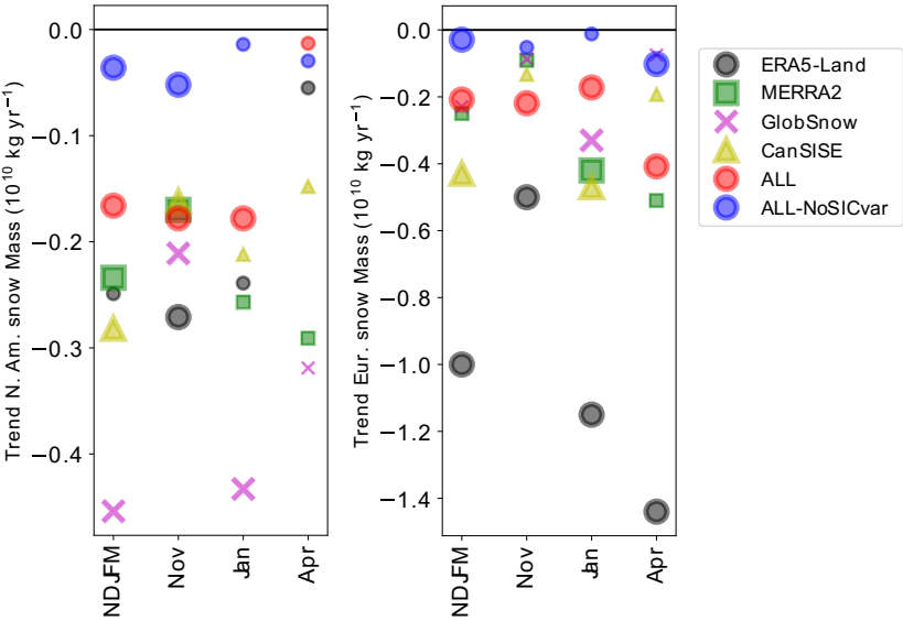
Figure S3: Same as Fig. S2, but for the Northern Hemisphere trend in snow mass, in 10 10 kg yr -1 with the ERA5-Land, MERRA2, GlobSnow and CanSISE data.
