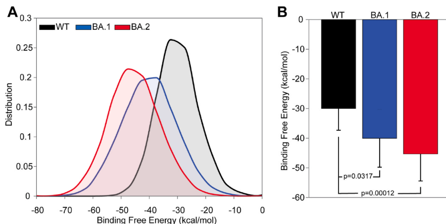
Fig. 4. Binding free energies of RBDs to PD. (A) Distribution of the binding free energies of RBD WT , RBD BA.1 , and RBD BA.2 . (B) Mean binding free energy values of the RBD WT , RBD BA.1 , and RBD BA.2 to PD. Error bars represent s.d. P values were calculated using a two-tailed Student's t-test.
