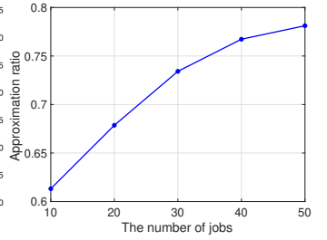
Fig. 7: Approximation ratio.
