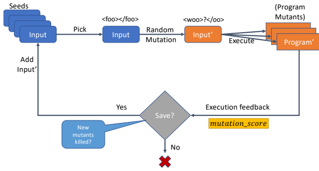
Figure 1: A mutation-analysis-guided fuzzing loop. Each fuzzer-generated input is run through a set of program mutants to compute a mutation score. Inputs are saved to the corpus if they improve mutation score.
