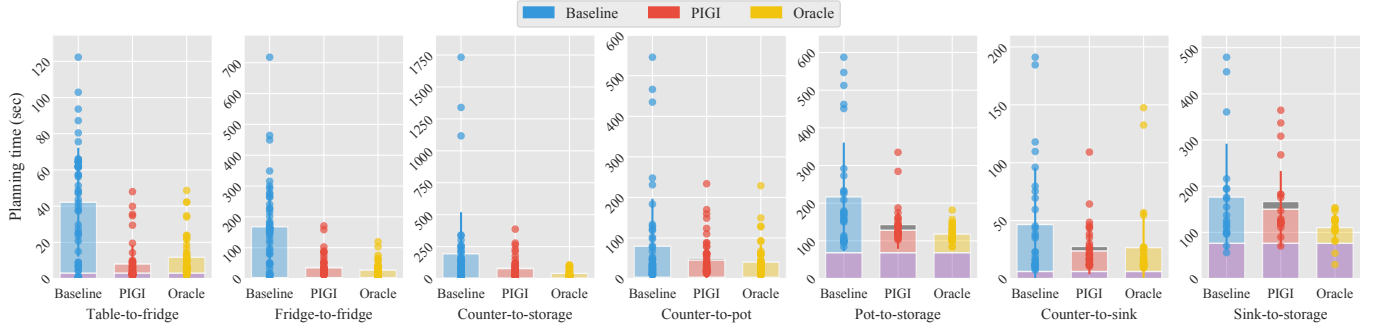
(a) The runtime breakdown of PIGINet-enabled planners compared to a non-learning Baseline and a clairvoyant Oracle. The purple bars indicate average task planning time by FastDownward for generating hundreds of candidate task plans in those problem sets. The gray bars indicate inference time running the candidate task plans through the PIGINet.
