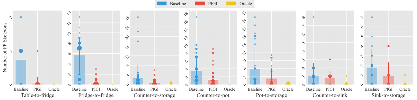
(b) The number of false positive (FP) task plans refined. The size of scattered dots are proportional to density.
