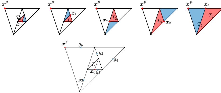
FIG 4. The chain of ancestors of E = T_0 leading to T_5 having a proper node as a vertex (above). The path g_1 \rightarrow g_2 \rightarrow \dots \rightarrow g_5 connecting \mathbf{x}_0 \in E to the proper node \mathbf{x}^P \in T_5 (below).
