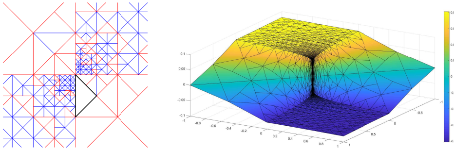
FIG 12. Test 2. Left: final grid \mathcal{T}_{VEM} , zoom to (-10^{-10}, 10^{-10})^2 (mesh elements having more than three vertices are drawn in red, and the mesh element drawn in black is a nonagon). Right: graph of the discrete solution.
