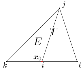
FIG 3. Sample of element E \in \mathcal{T} , where T = A(E) is the parent of E ; i, j, k are the global indices of the vertices of E ( i being the global index of \mathbf{x}_0 ); and \ell is global index of the remaining vertex of T .
