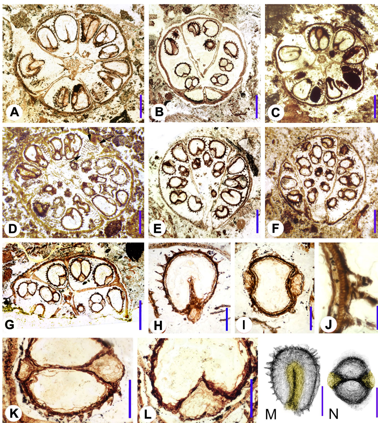
Figure 1. Surangea mohgaonensis fruits and seeds. A–L. Acetate peel sections by combined reflected and transmitted light microscopy; A–C. Specimens from Mohgaonkalan; A. Transversely sectioned fruit showing thick pentagonal central axis and thin radial septa delimiting five locules, containing seeds with their narrow hilar ends facing inward, indicating axile placentation, UF 18311-62124; B. Holotype, peel cutting obliquely through five locules, delimited by narrow septa, CMNH PM-1388; C. Transverse section showing central vasculature and five locules, UF 18311-62124; D. Specimen from Paladaun, peel intercepting seeds at various levels. Note tangential section of seed coat periphery with ridged ornamentation appearing as parallel lines (upper right). UF 19506-70519; E. Specimen from Mohgaonkalan, UF 18311-70429; F. Obliquely sectioned fruit from Keria, UF 19329-62155; G. Section at level showing more clearly the five locules from Mohgaonkalan, UF 18311-62123; H–L. Details of individual seeds from Keria, UF 19329-62155; H. Single seed in lateral section showing curved cavity and basal aril; I. Seed in transverse section showing central cavity and peripheral aril; J. Detail of seed coat; K, L. Detail of seeds showing large cells composing the aril; M, N. Seed reconstructed in 3D, digitally extracted from micro-CT data from the specimen in F; surface rendering in lateral and apical views with translucency; aril shaded yellow. Scale bars = 1 mm in A–G; 250 \mu m in H, I, K–L; 100 \mu m in J, 500 \mu m in M, N
