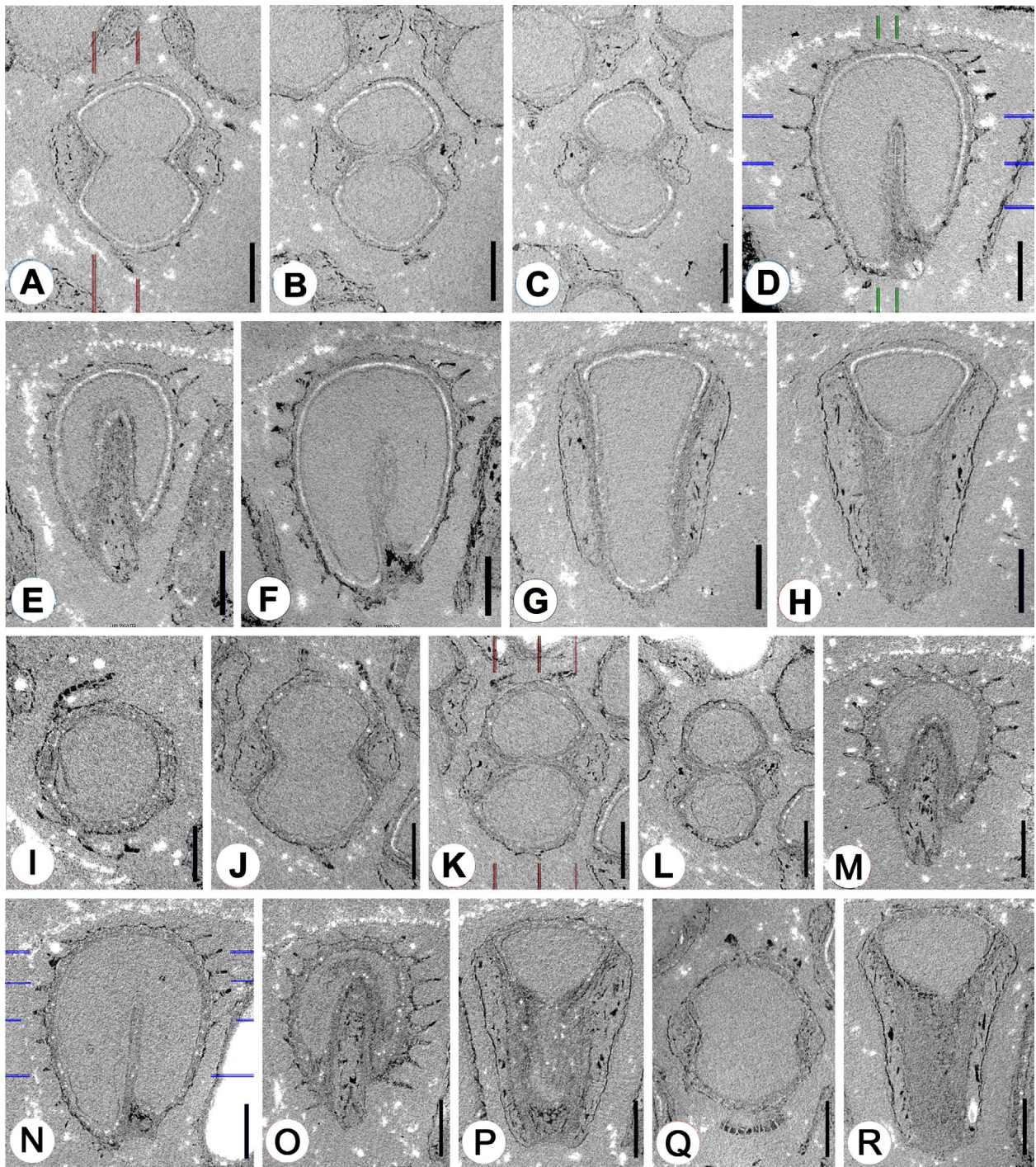
Figure 3. Surangea mohgaonensis seeds in digital section from micro-CT scan of a fruit from Keria, UF 19329-62155 (same specimen as Fig. 2H–Y). A–H. Seed “d” in transverse (A–C), sagittal (D–F) and coronal (G, H) sections. Registration lines in A and D show the planes of section represented in E, F and A–C, G, H, respectively; I–P. Seed “e” in transverse (I–L), sagittal (M–O) and median coronal (P) section. Registration lines in K and N show the planes of section represented in figures M–O and I–L, respectively; Q, R. Seed “f” in transverse section at apical one-third showing ornamentation of seed coat (Q), in median coronal section (R), intercepting the aril on both lateral margins. Scale bars = 0.25 mm
