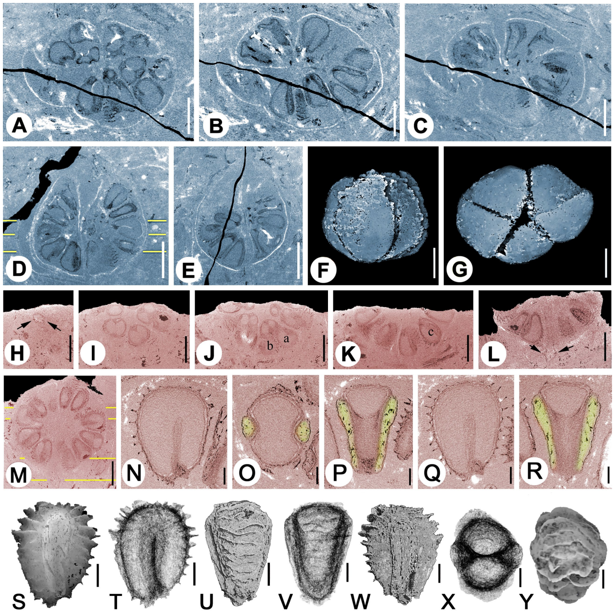
Figure 2. Surangea mohgaonensis fruit and seeds. Virtual serial sections and extracted seed from micro-CT scan data. A–G. Fruit from Mohgaonkalan, UF18311-19116; A–C. Successive transverse sections moving apically according to registration lines in D , showing thin fruit wall, and seeds in apparent axile placentation; D, E. Longitudinal sections at right angles to one another; F, G. Lateral and basal views of the pentacarpellate septicidal capsule, digitally extracted from the chert, depth map rendering; H–Y. Specimen from Keria; same as that shown by light microscopy (Fig. 1F, H–L), UF 19329-62155; H–K. Successive transverse sections arranged from pedicel ( H , arrows), near base ( I ), slightly above equator ( J ) to apical one third ( K ) at levels indicated in M showing the organization of seeds within each of the locules; seeds labeled “a–c,” are enlarged in N–Y ; L. Median longitudinal section in plane of the pedicel (arrows) and central axis; M. Median longitudinal section at right angles to the plane of L , with registration lines indicating the planes of H–K ; N–P. Seed “a” in sagittal, transverse and coronal section, aril indicated in yellow; Q, R. Seed “b” in sagittal and coronal section, aril indicated in yellow; S–Y. Seed “c,” digitally extracted showing surface sculpture by depth map rendering ( S, Y ), opaque surface rendering ( U, W ) and translucent surface rendering ( T, V, X ), rotated through sagittal ( S, T, W ), coronal ( U, V ) and apical ( X, Y ) orientations. Scale bars = 1 mm in A–M , 0.2 mm in N–Y
