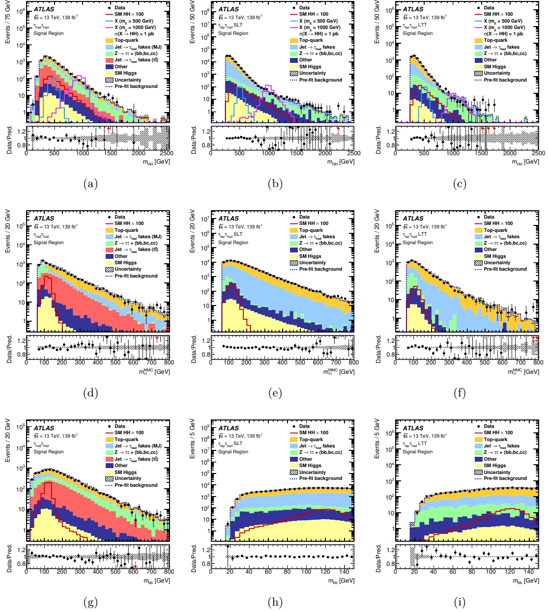
Figure 3. Signal (solid lines), background (filled histograms) and data (dots with error bars) distributions of m_{HH} (top), m_{\tau\tau}^{\text{MMC}} (middle row) and m_{bb} (bottom) for events in the \tau_{\text{had}}\tau_{\text{had}} (left), \tau_{\text{lep}}\tau_{\text{had}} SLT (middle column) and \tau_{\text{lep}}\tau_{\text{had}} LTT (right) categories. The normalisation and shape of the backgrounds and the uncertainty in the total background shown are determined from the likelihood fit (described in section 8) to data in the non-resonant HH search. The expected non-resonant signal is overlaid with its normalisation scaled by a factor of 100, and the m_X = 500 GeV and m_X = 1000 GeV resonant signals are overlaid in the m_{HH} distributions with their cross-section set to 1 pb. The dashed histogram shows the total pre-fit background. The size of the combined statistical and systematic uncertainty of the background is indicated by the hatched band. The ratio of the data to the sum of the backgrounds is shown in the lower panels.
