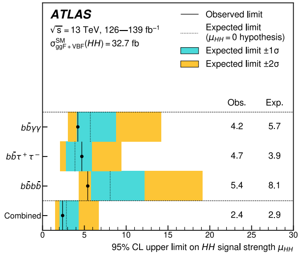
Fig. 3. Observed and expected 95% CL upper limits on the signal strength for double-Higgs production from the bbbb , bb\tau^+\tau^- and bb\gamma\gamma decay channels, and their statistical combination. The value m_H = 125.09 GeV is assumed when deriving the predicted SM cross-section. The expected limit and the corresponding error bands are derived assuming the absence of the HH process and with all nuisance parameters profiled to the observed data.
