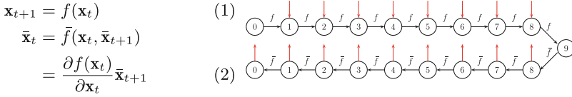
Fig. 2. Evaluation process of iteratively applying function f for t = 1 : 9 iterations, f is called with state x_t as the input and state x_{t+1} as the output. The adjoint function \bar{f} of f computes state \bar{x}_t with respect to state \bar{x}_{t+1} and x_t . The red down and up arrows mark a stored and restored state, respectively.
