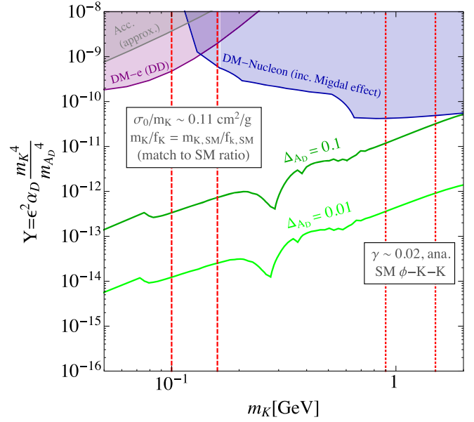
FIG. 2. The most motivated mass ranges for resonant self-interaction, analogous to the \phi - K - K system discussed in the text, are enclosed by red dashed and dotted lines. The green curves give the correct relic abundance with \Delta_{A_D} = (m_{A_D}^2 - 4m_K^2)/4m_K^2 = 0.1 and 0.01 , reproduced from Ref. [51]. The purple regime is constrained by DM-electron direct detection; the gray regime is the approximate accelerator bound (see text for discussions), and the blue region is constrained by the DM-nucleon scattering (including the Migdal effect).
