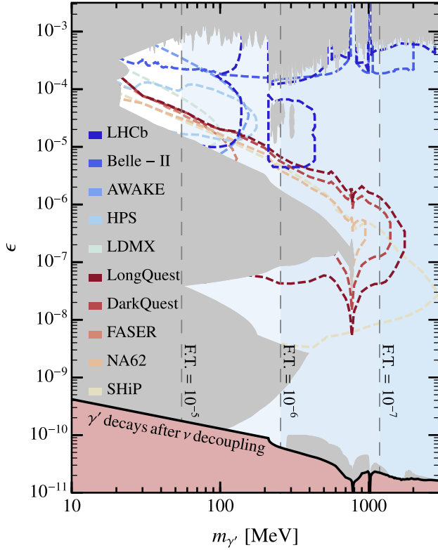
FIG. 4. The parameter space in the heavy quark model in which the dark photon decays quickly enough to transfer the dark \pi 's entropy before neutrino decoupling. Existing constraints [82–91] are dark gray while projected sensitivities of future experiments are shown as dashed lines [83,91–104]. The dashed vertical lines show different levels of accident (F.T.) required to achieve the necessary resonant self interaction, as defined in Eq. (13).
