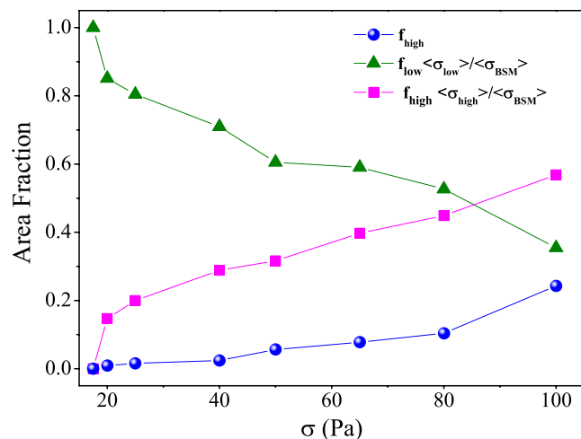
Fig. 3. High-stress fronts are responsible for shear thickening. The area fraction of the stress maps containing high stresses (blue circles) is negligible at applied stresses at or below \sigma_c , but rises rapidly with applied stress, reaching over 20% of the area at 100 Pa. The stress contribution from the high-stress regions (magenta squares) grows as the applied stress is increased at the expense of the contribution from the low-stress regions (green triangles) until it becomes the dominant source of stress. \phi_w = 42.3\% .
