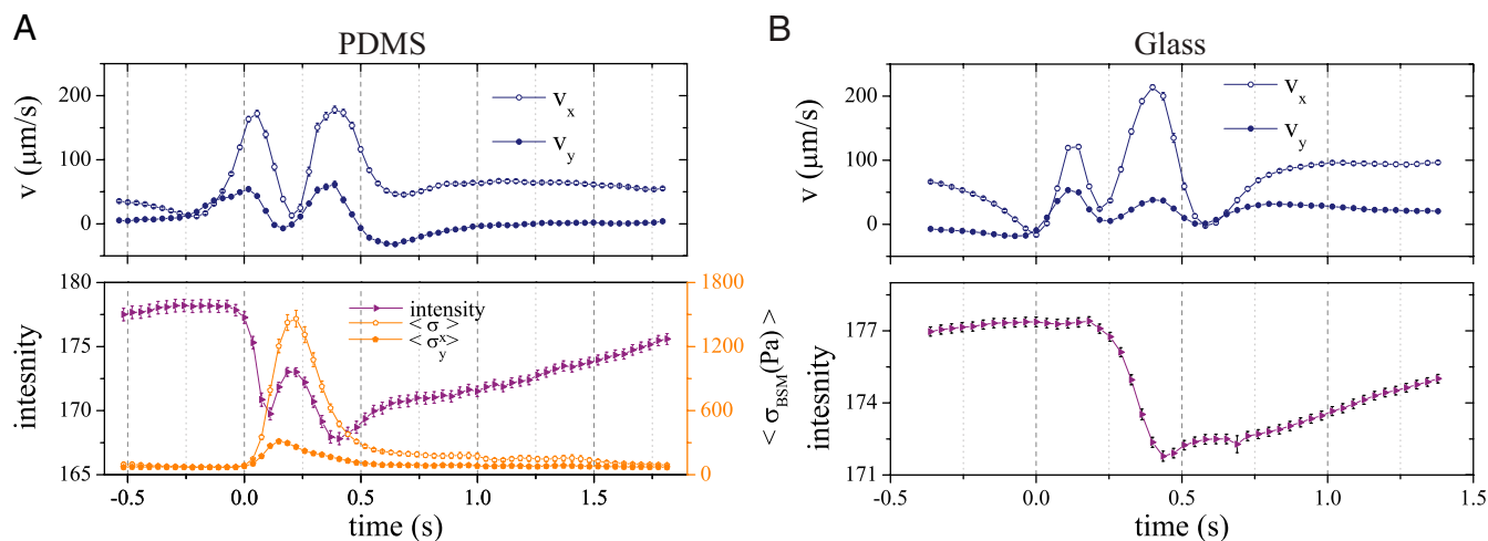
Fig. 6. Average event shape for (A) PDMS-coated bottom surface and (B) uncoated glass. v_{xy} represents the components of the velocity of the bottom layer of cornstarch particles in the flow and vorticity directions, respectively, measured by PIV (as in Fig. 4), while \langle \sigma_{xy} \rangle shows the image-averaged components of the boundary stress. The intensity values, calculated directly from the images of the cornstarch particles, provide a measure of the cornstarch concentration in the bottom layer.
