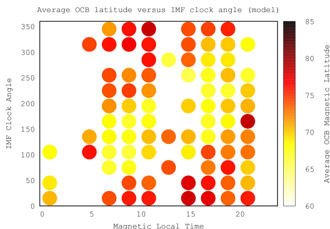
Figure 13. Average MLAT (over all events) as a function of MLT and CLK for the OpenGGCM results.
