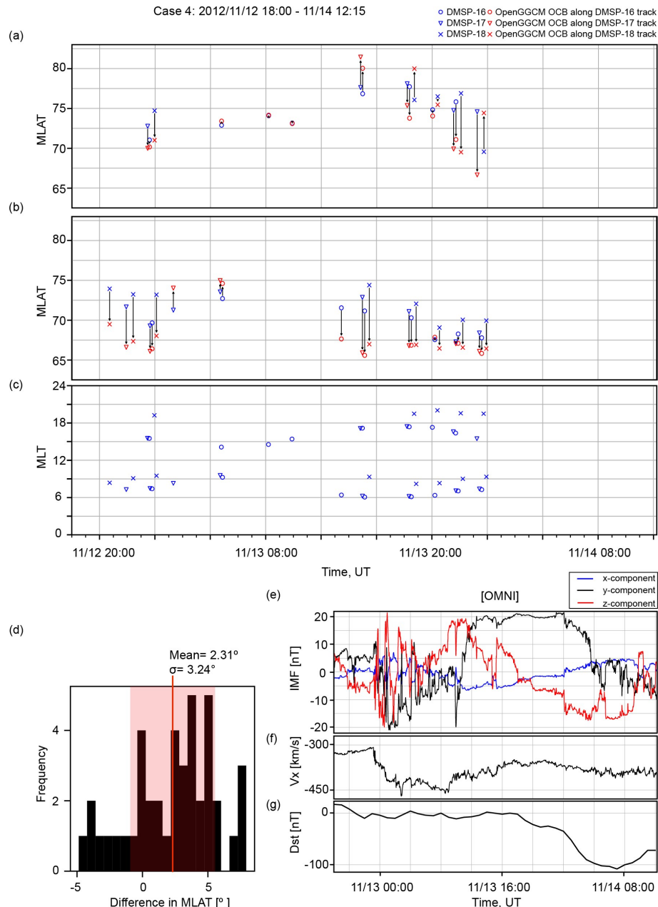
Figure 4. Comparison between the observed and simulated OCB latitudes for 13 November 2012 event in the same format as Fig. 1.
