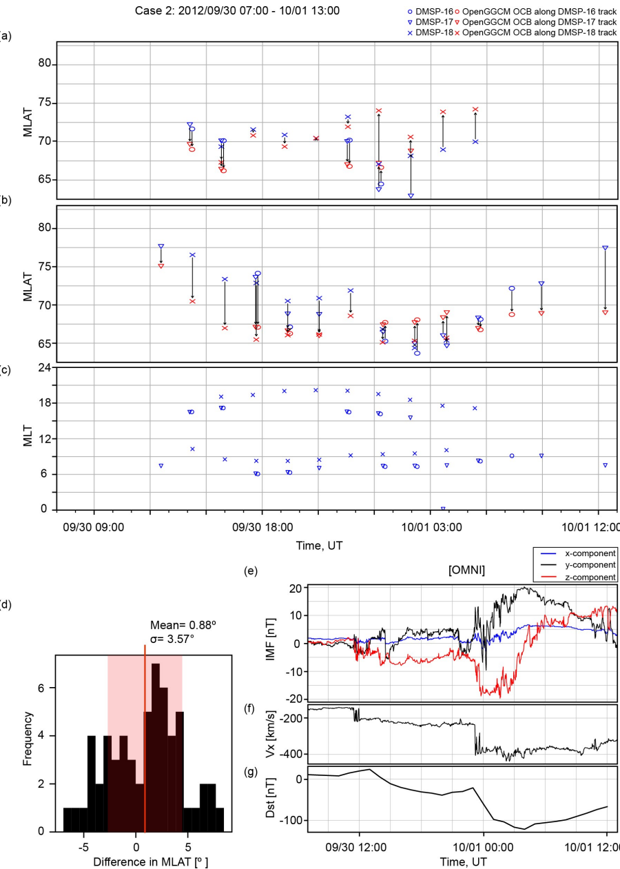
Figure 2. Comparison between the observed and simulated OCB latitudes for the 1 October 2012 event in the same format as Fig. 1.
