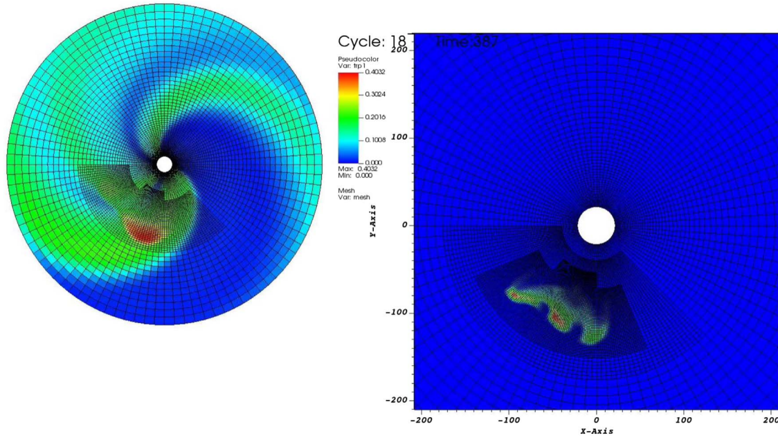
Fig. 9. Left: snapshot of a two-level solution adapted mesh for a cone CME in a stretched grid using TVDLF. Right: another example snapshot of a different test with three levels of AMR.
