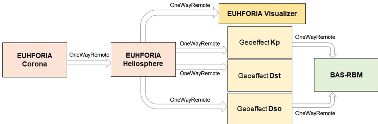
Fig. 1. One of the Sun-to-Earth modelling chains implemented in the VSWMC that became operational in 2019 (see Poedts et al., 2020). In this chain EUHFORIA is coupled to models to determine the Kp and Dst indices and the plasma sphere stand-off distance, based on the synthetic wind data at L1 from EUHFORIA. The Kp index and the plasma sphere stand-off distance (Dso) are then used to drive the British Antarctic Survey Radiation Belt Model.
