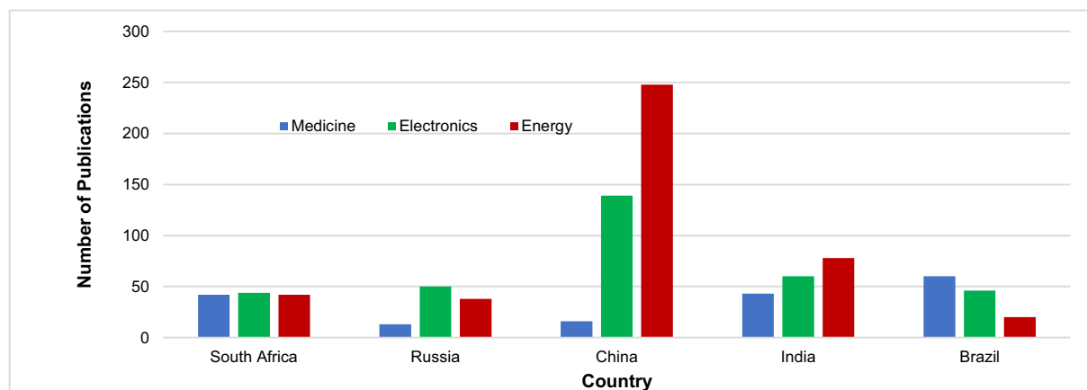
Fig. 8 South Africa publications reporting on nano-enabled products relative to BRICS countries
