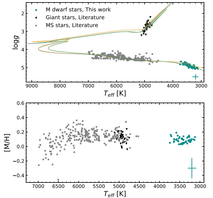
Figure 4. Top panel: a Kiel diagram showing the results for the Hyades M dwarfs obtained here from APOGEE spectra (cyan circles), along with those from high-resolution optical studies from the literature for Hyades FGK dwarfs (gray Xs) and red giant stars (black triangles). Three sets of isochrones with an age of 0.6 Gyr are shown as guidelines: PARSEC (V2.0; yellow line, [M/H] = +0.07 ), DARTMOUTH (gray line, [M/H] = +0.07 ) and MIST (green line [M/H] = +0.1 ). Bottom panel: comparisons between the metallicities vs. T_{\text{eff}} for the M dwarfs (this work), along with those from red giants and hotter dwarfs from the Hyades cluster, with these comparisons spanning almost 4000 K in T_{\text{eff}} . The median metallicity for the M dwarfs studied here is \langle [M/H] \rangle = 0.09 \pm 0.03 , and shows no significant trend as a function of T_{\text{eff}} ; it is also in good agreement with the median metallicity for the red giants from the literature ( \langle [M/H] \rangle = 0.12 \pm 0.03 ). The literature results reveal a dip in metallicity for the hotter dwarfs with effective temperatures between 6000 and 7000 K. The estimated uncertainties are shown as error bars.
