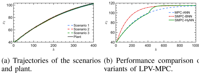
Fig. 4. Validation of the proposed SMPC scheme.
