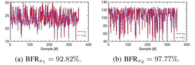
Fig. 2. Validation of the nominal LPV-ANN model.
