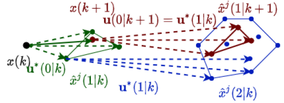
Fig. 1. Recursive feasibility.
