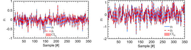
Fig. 3. Validation of the BNN-based mismatch model.
