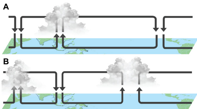
Figure 4. Schematic of the Indo-Pacific Walker Circulation change. Conditions when (A) C_3 plants dominate pre-250 ka glacial and all interglacials, and (B) C_4 plants dominate glacial after 250 ka.
