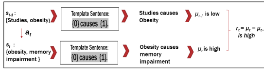
Fig. 2. Scoring method explained for the sentence “Studies have supported that obesity accelerates AD-related memory impairment.” using question templates
