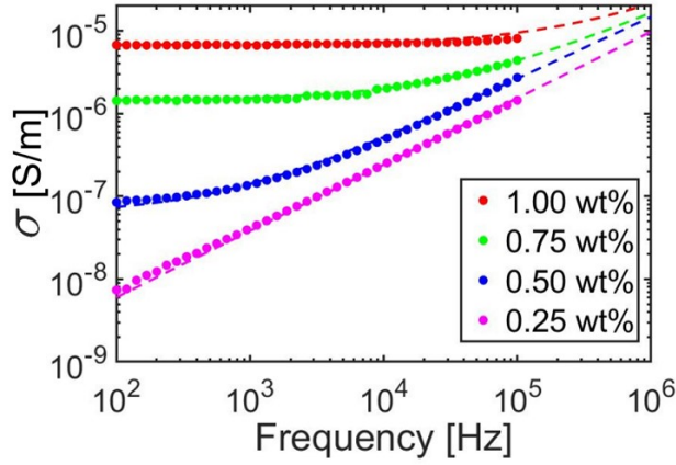
Fig. S 1: PNC conductivity vs. AC frequency with different CNT doping ratios: markers are experimentally measured and dashed lines are fitted using Eq. 1.
