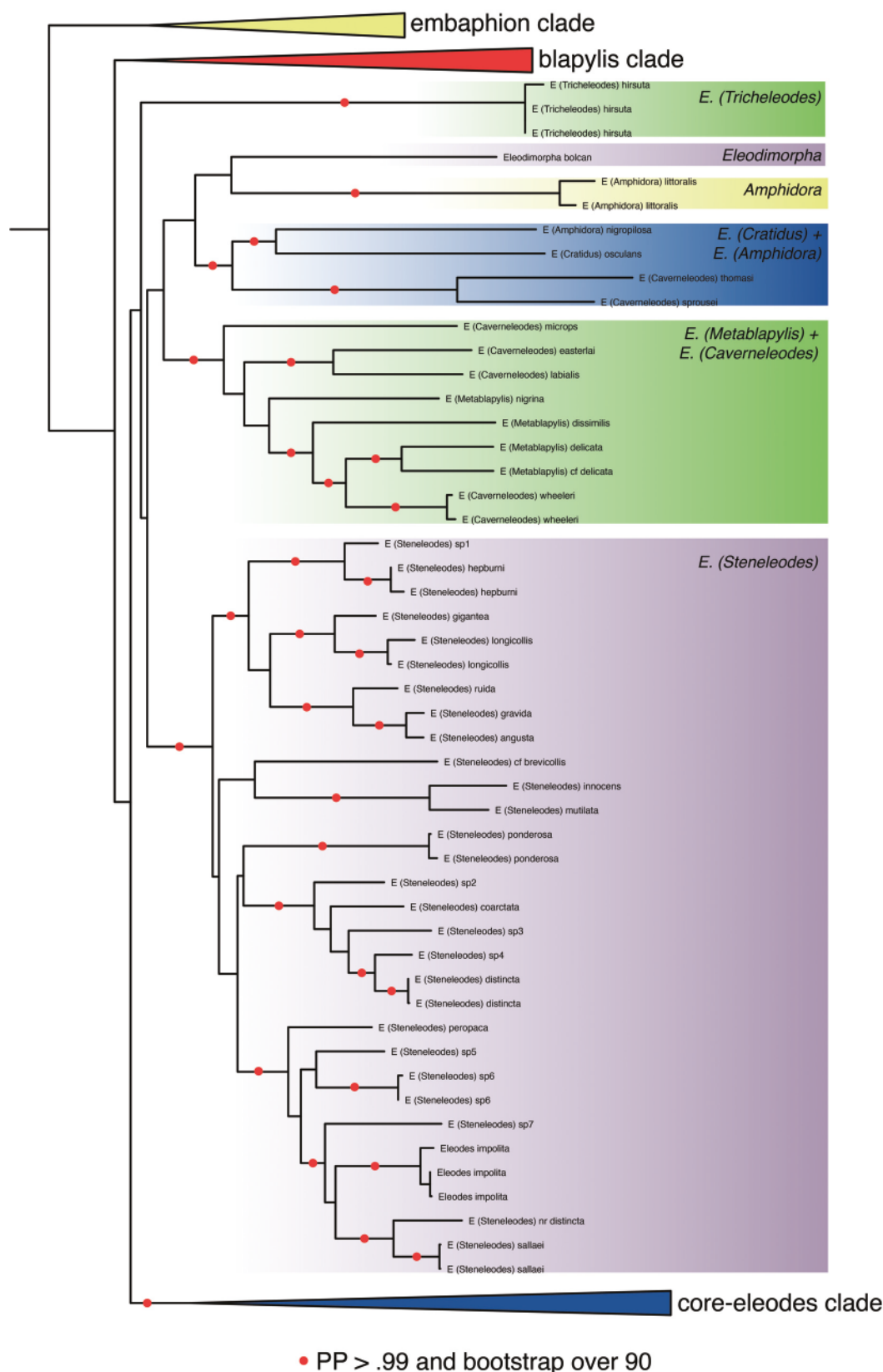
Figure 3. Among-Amphidorini phylogeny continued. Topology shown is the same as Fig. 2 with the metablapyllis group expanded. Branches marked with a red dot were recovered in both Bayesian inference and maximum likelihood analyses with at least .99 posterior probabilities and 90 bootstrap values, respectively.
