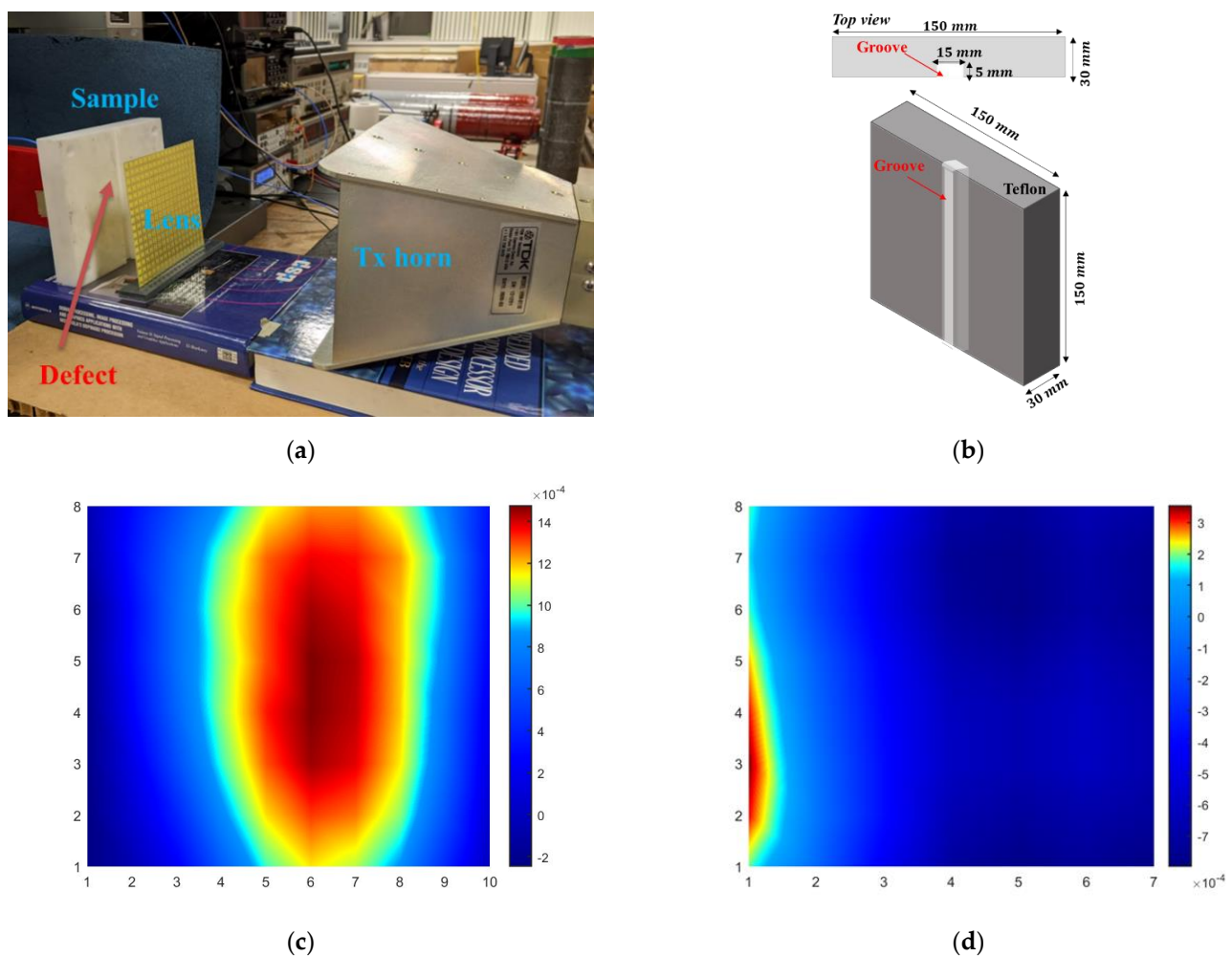
Figure 11. (a) Microwave NDE experiment setup. (b) Schematic of Teflon sample under test with machined groove. (c) Microwave imaging results of groove defect with lens and (d) without lens.
